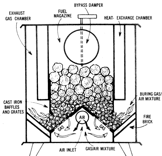
Fig. 15. Draft-flow pattern in Downdrafter box stove.
