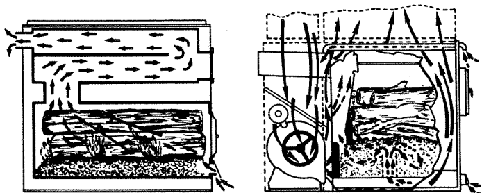
Fig. 80. Valley Comfort wood-burning furnace flow-patterns.
