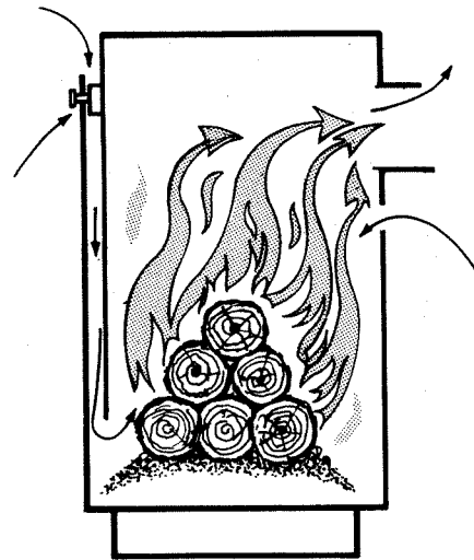
Fig. 10. Draft-flow pattern of the Ashley stove.
