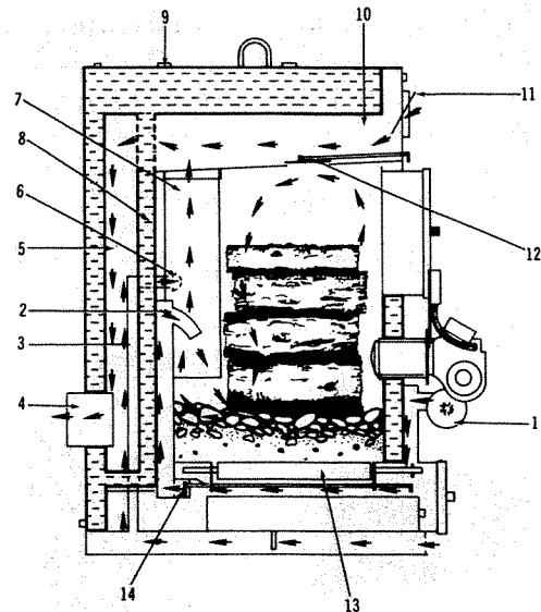
Fig. 87. Riteway boiler.
