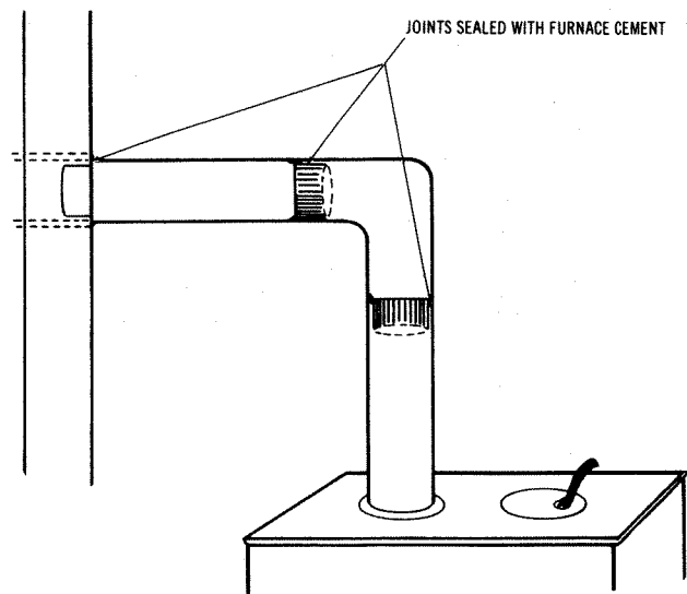
Fig. 4. Seal all stovepipe joints with furnace cement. Note that female ends of pipes face the chimney.
