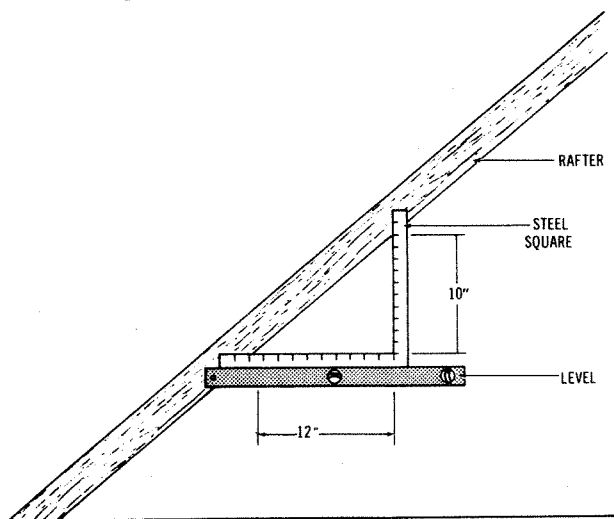
Fig. 8. Measuring roof pitch, using level and steel square.
