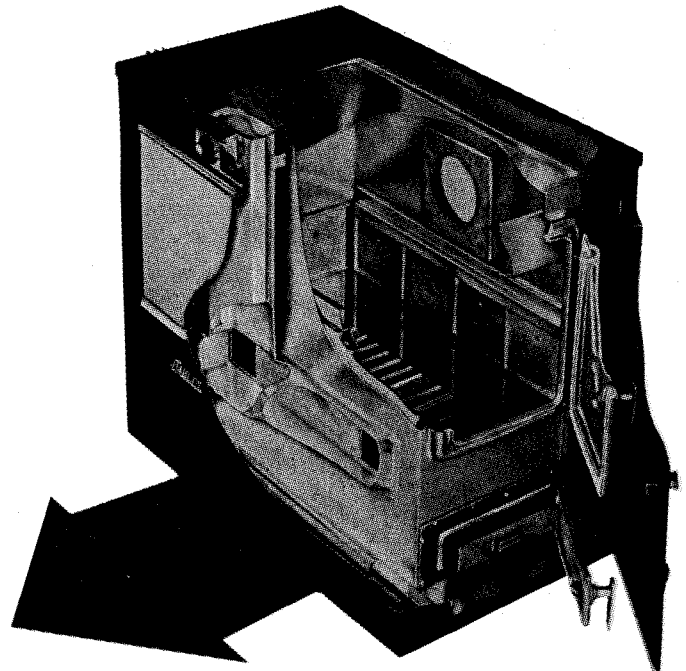
Fig. 22. Cutaway view of Ashley circulating heater, showing interior construction.
