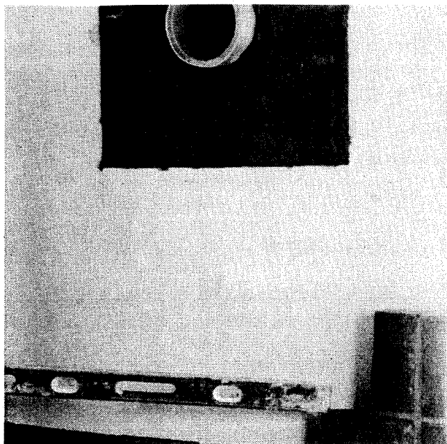
Fig. 16. Interior view after bricking-in, showing thimble (at top) and start of header course of hearth wall.
