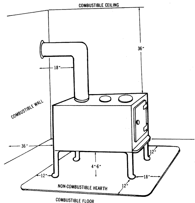
Fig. 1. Suggested minimum clearances from combustible surfaces.
