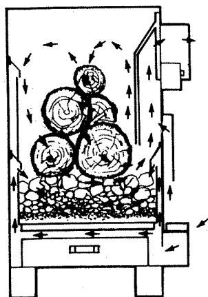
Fig. 11. Air-flow pattern in the Riteway 2000.
