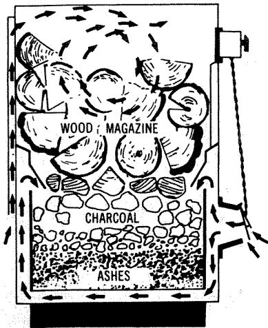
Fig. 25. Valley Comfort automatic circulating heater, showing flow-patterns.
