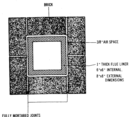
Fig. 13. Top view of chimney, showing wall brick, flue liner, and air space between liner and chimney wall.
