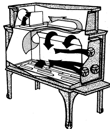
Fig. 8. Cutaway view of Nordic stove with flip-open damper and contoured side baffles.
