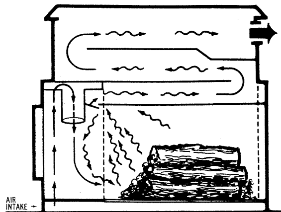
Fig. 6. Flow-pattern and baffle arrangement in Home Warmer stove.
