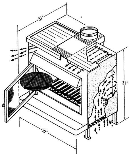
Fig. 45. The Impression 5 freestanding fireplace/stove.
