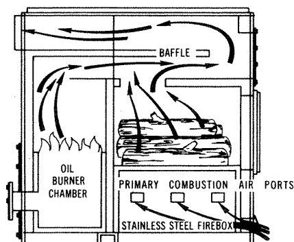
Fig. 79. Hunter combination wood/oil furnace flow-patterns.
