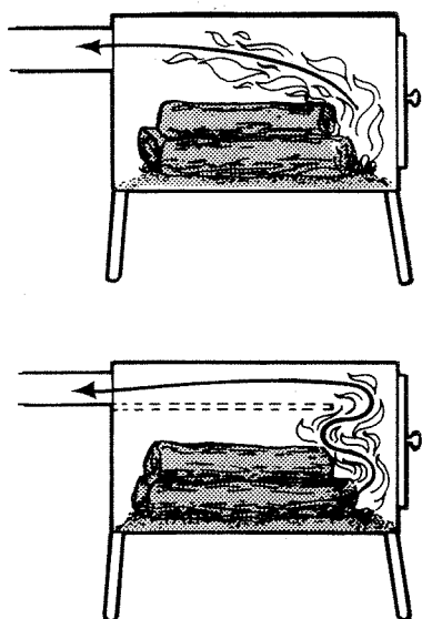
Fig. 2. Direct flame-path in traditional box stove versus "S"-shaped flame-path in Scandinavian baffled stove.
