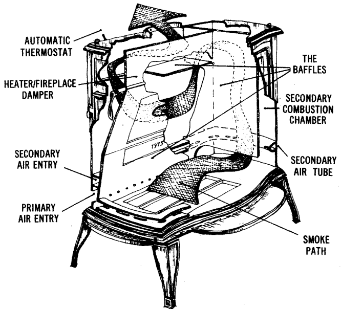
Fig. 12. Cutaway view of the Defiant stove.
