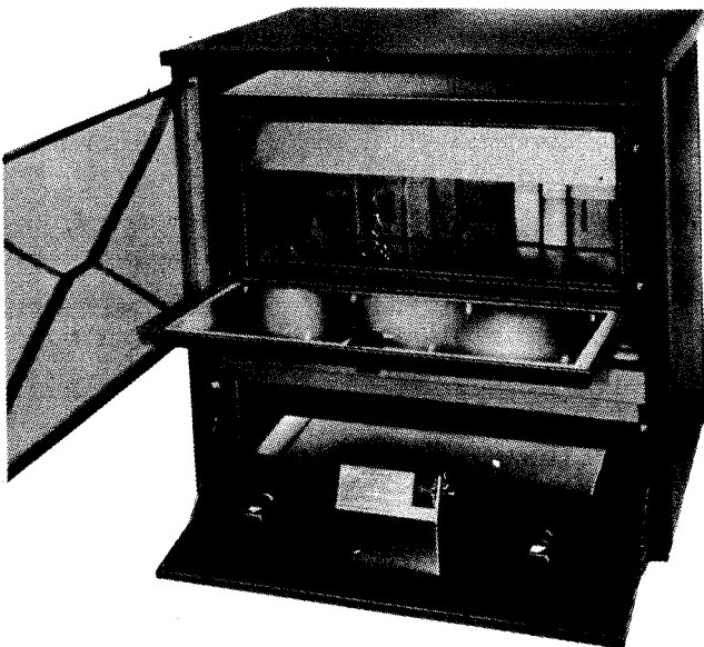
Fig. 24. Autocrat Model FF76 automatic circulating heater.
