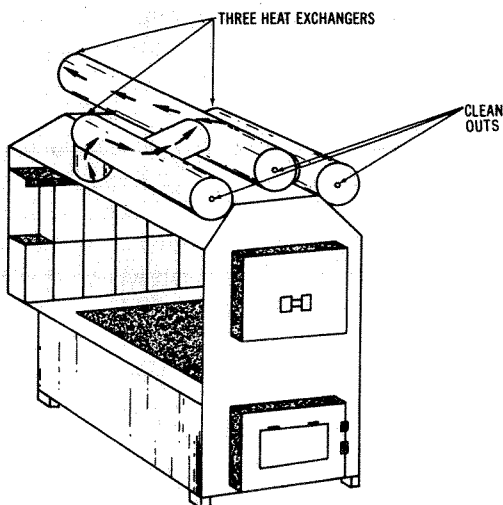
Fig. 82. Ray-Mask wood-burning furnace.
