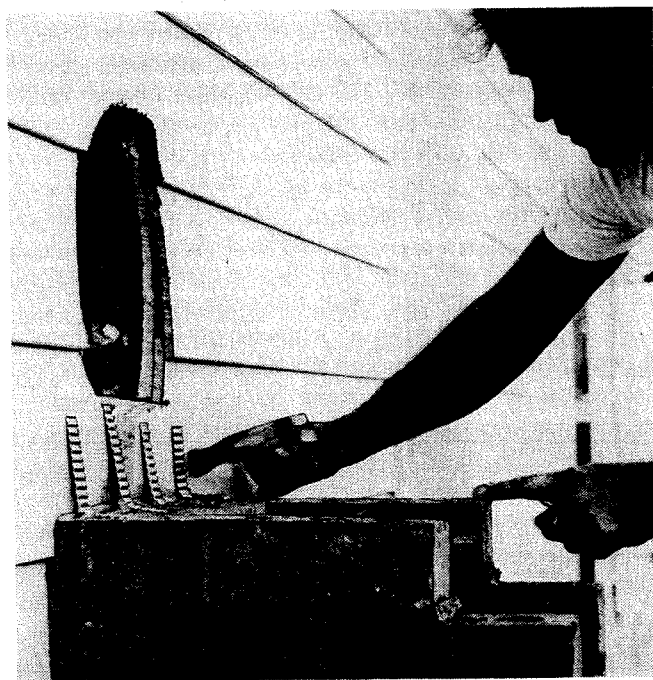
Fig. 14. Corrugated steel wall ties placed every sixth course of brick.
