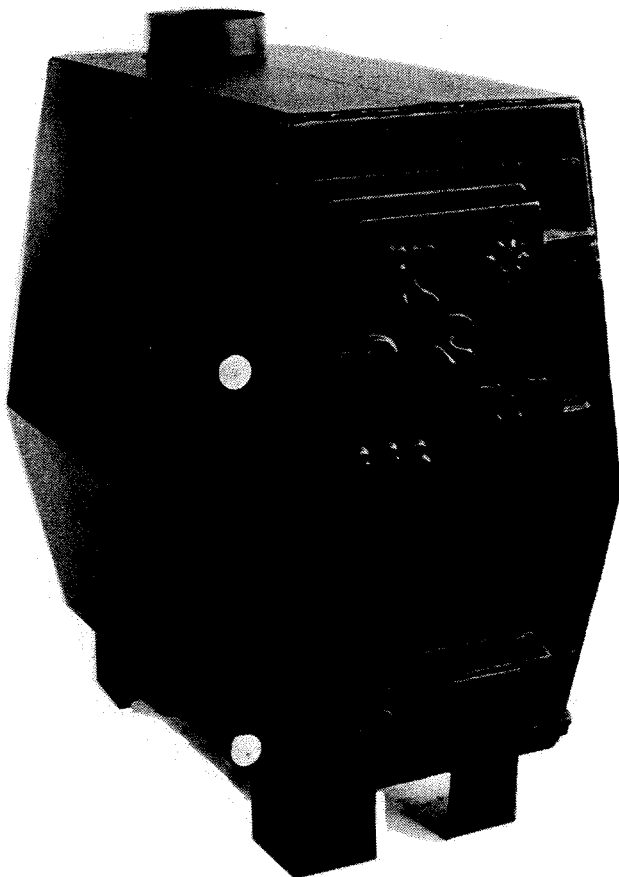
Fig. 73. Kickapoo Standard Model BBR-B wood-burner.
