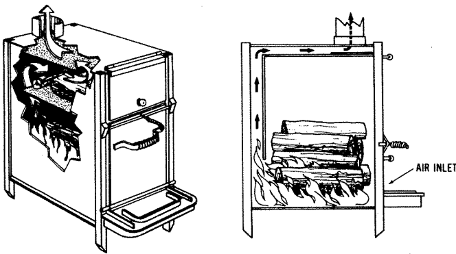
Fig. 63. Greenwood (left) and Double Dynamite (right).
