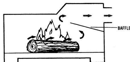
Fig. 47. Flow-pattern and baffle in the Alaskan.
