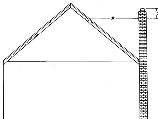
Fig. 5. Chimney height in relation to 10-foot distance from roof.
