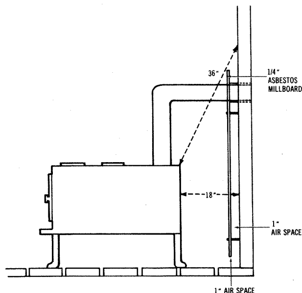
Fig. 2. Suggested minimum clearances from protected combustible walls.
