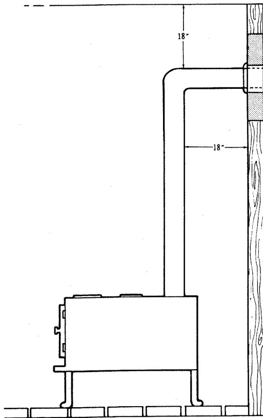
Fig. 3. Suggested minimum clearance of stovepipe from combustible surfaces.
