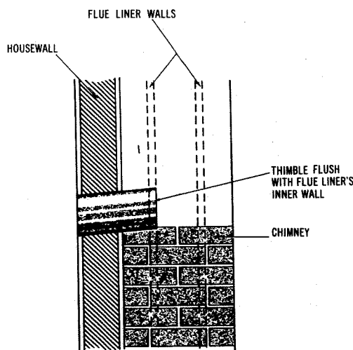
Fig. 18. Position of thimble with respect to wall of flue liner.
