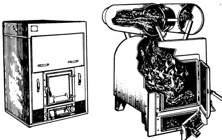
Fig. 77. Daniels wood-burning furnace (left) showing interior view (right).
