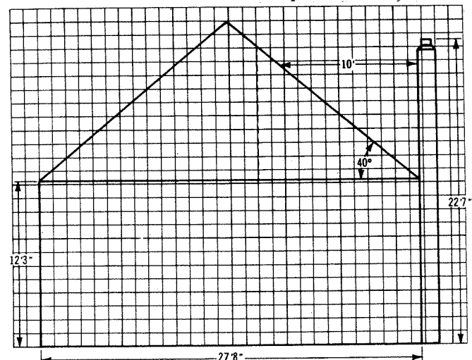
Fig. 9. Transferring data to graph paper for a scale drawing.
