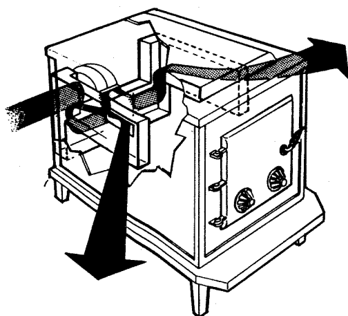
Fig. 7. Heat manifolds used in Nashua stove.
