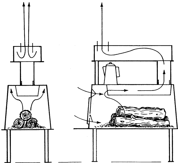
Fig. 5. Front and side views of Solis 6 stove.
