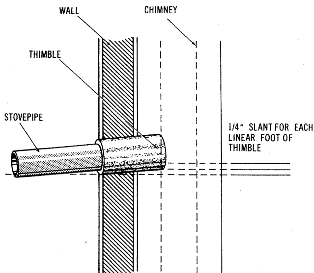
Fig. 17. Angle of thimble from horizontal.
