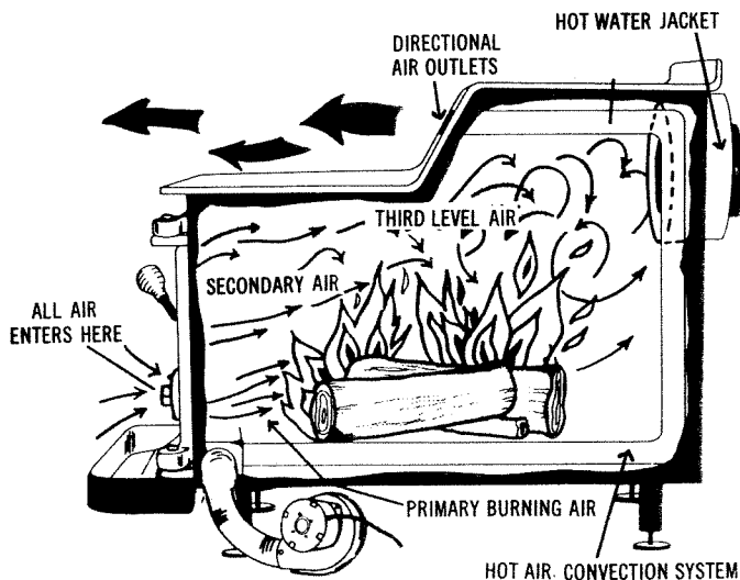
Fig. 13. Cutaway of All Nighter step stove.
