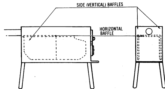
Fig. 1. Scandinavian woodstove interior baffle arrangement from side (left) and front (right).
