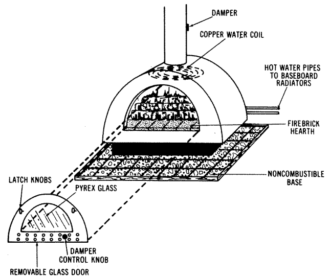
Fig. 44. Greenbriar freestanding fireplace/stove.
