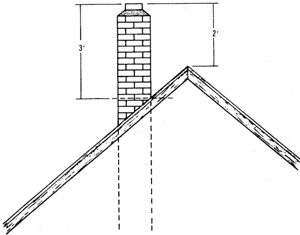
Fig. 3. Height of chimney above roof and ridge.
