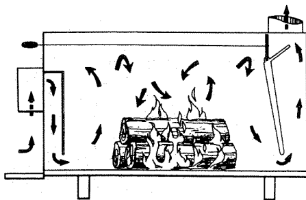
Fig. 67. Thermo-Control's heat-flow pattern.
