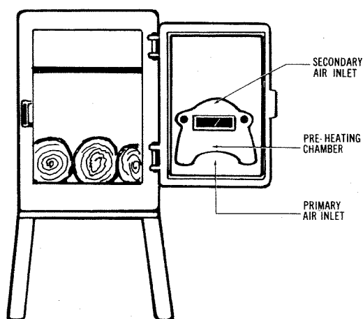
Fig. 3. Preheating chamber with primary and secondary air inlets.
