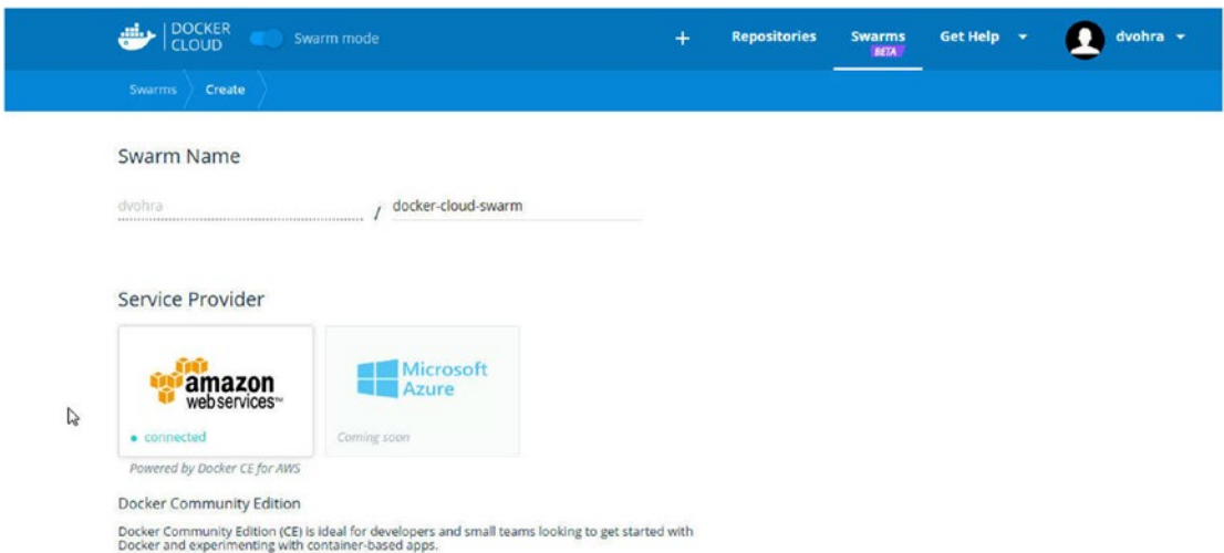
Figure 14-29. Creating a Docker Swarm using the AWS service provider
