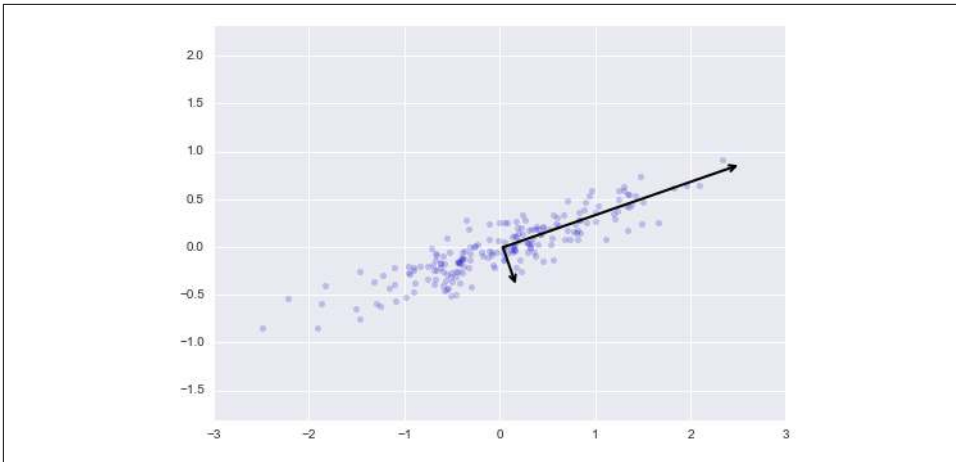
Figure 5-81. Visualization of the principal axes in the data
