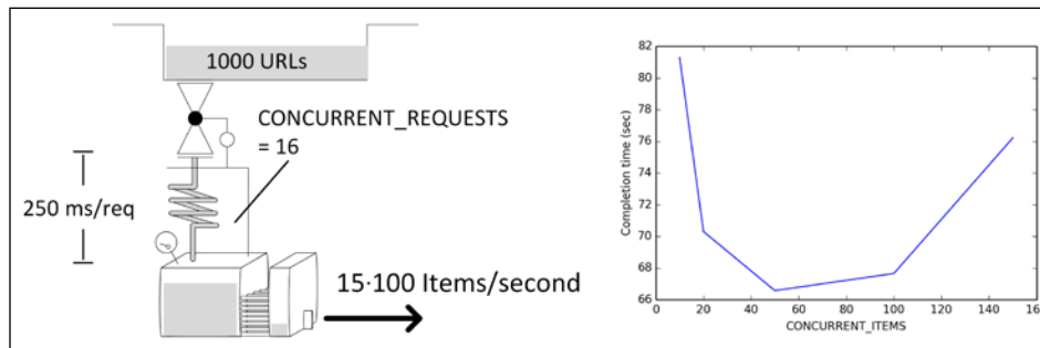
Figure 11. Crawl time as a function of CONCURRENT_ITEMS
