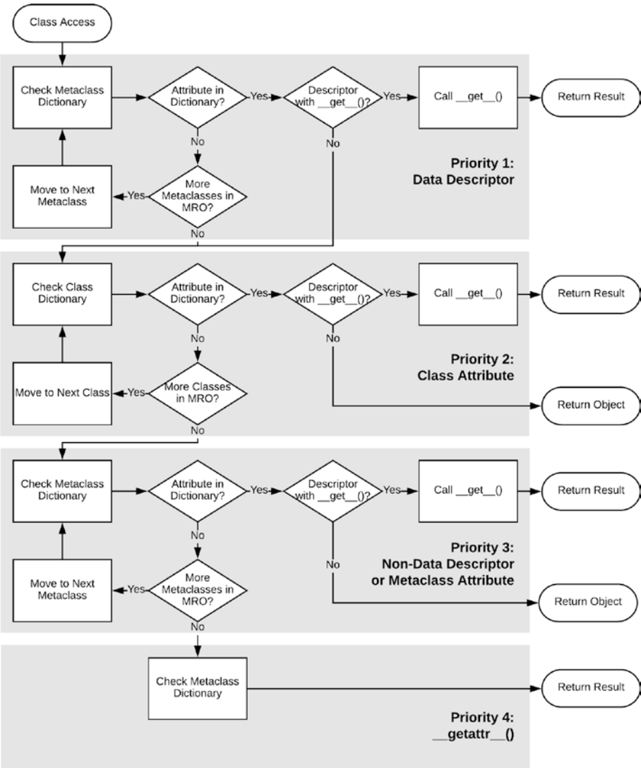
Figure 5-3. The full class access diagram
