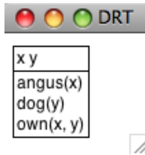
Figure 5.2: DRS Screenshot
