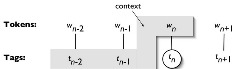
Figure 5.1: Tagger Context
