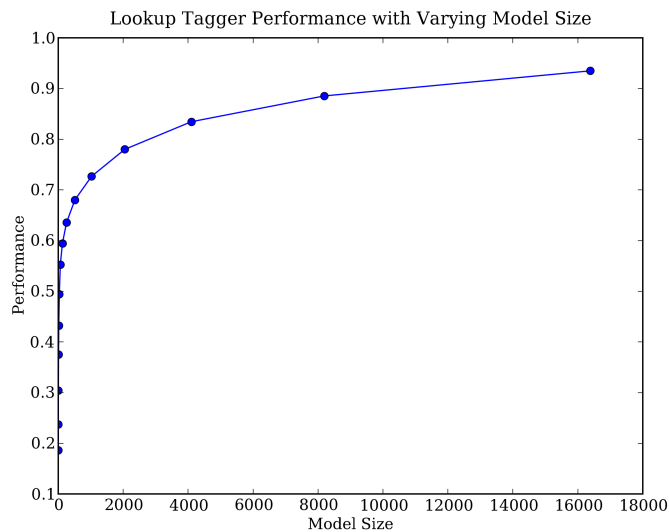
Figure 4.2: Lookup Tagger
