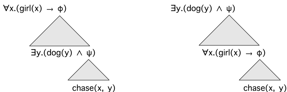
Figure 4.1: Quantifier Scopings
