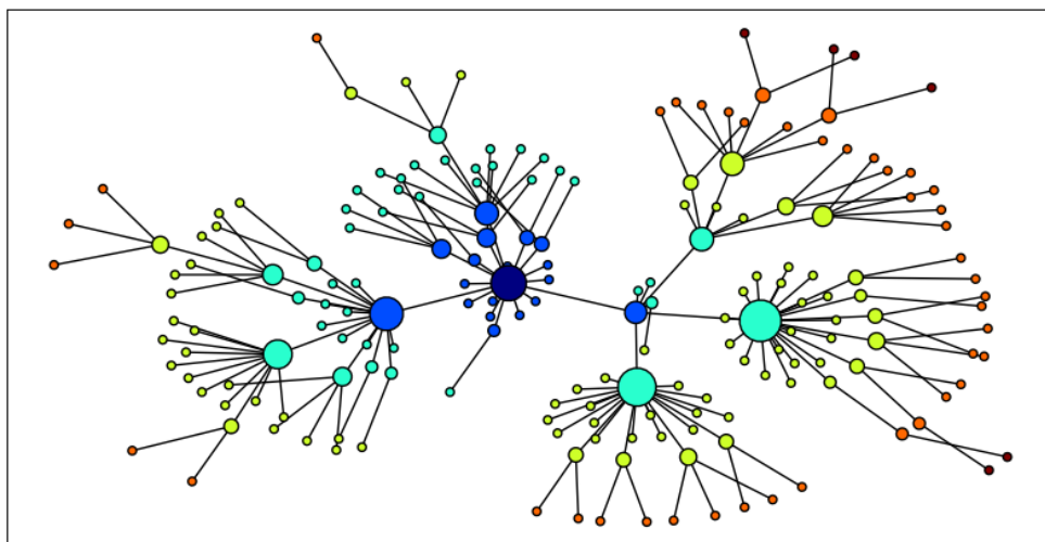
Figure 4.16: Visualization with NetworkX and Matplotlib: Part of the WordNet hypernym hierarchy is displayed, starting with dog.n.01 (the darkest node in the middle); node size is based on the number of children of the node, and color is based on the
