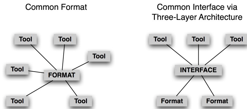
Figure 3.2: A Common Format vs A Common Interface
