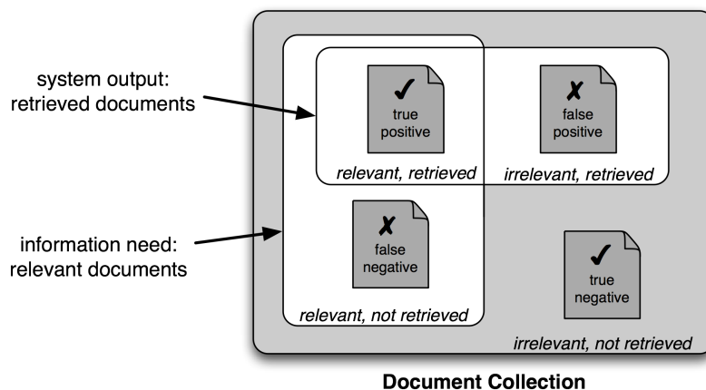
Figure 3.1: True and False Positives and Negatives
