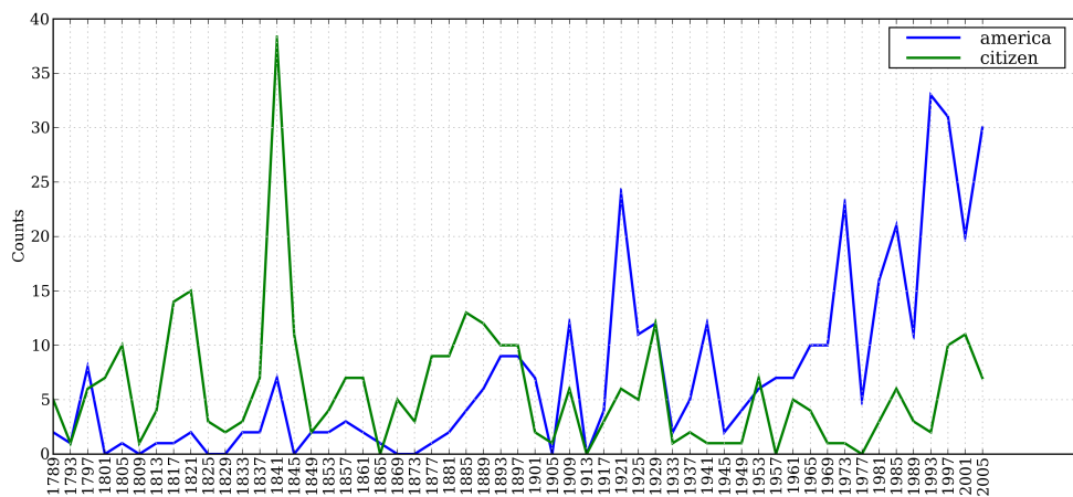
Figure 1.1: Plot of a Conditional Frequency Distribution: all words in the Inaugural Address Corpus that begin with america or citizen are counted; separate counts are kept for each address; these are plotted so that trends in usage over time can be observed; counts are not normalized for document length.
