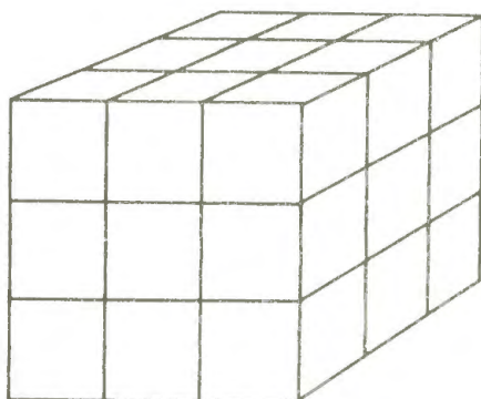
3 cubed, or 3^3
