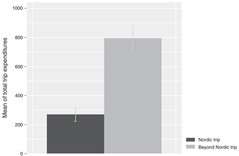
Figure 6.9 Means and 95 percent CIs for total trip expenditures by trip destination.
