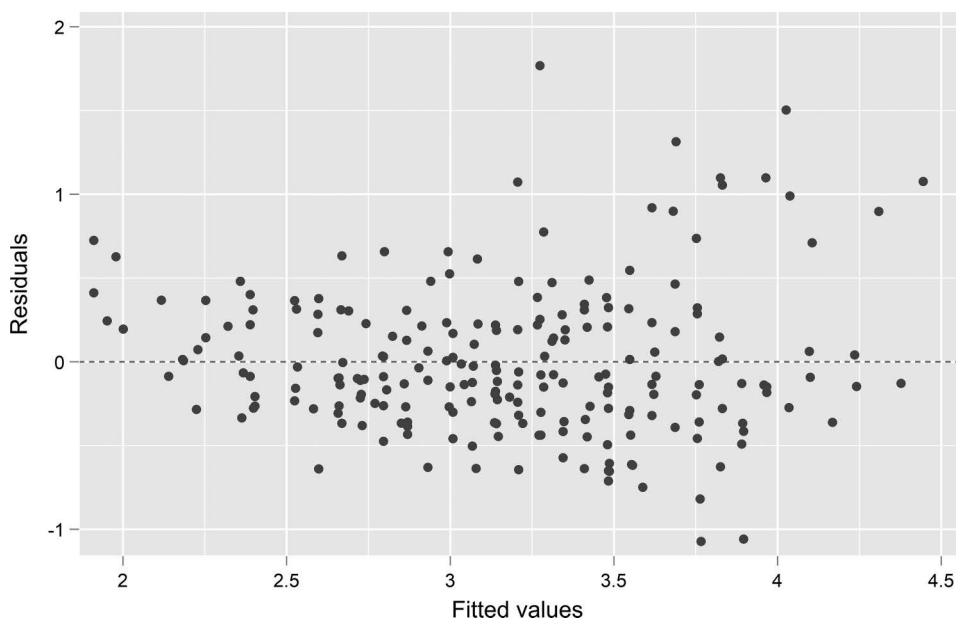
Figure 6.12 Residuals-versus-predicted/fitted-values plot.
