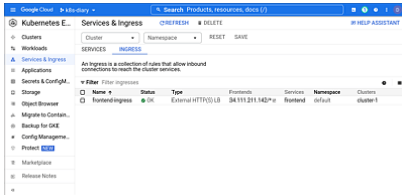
Figure 20.11 Kubernetes Ingress Services for the Diary Example in the Google Cloud
