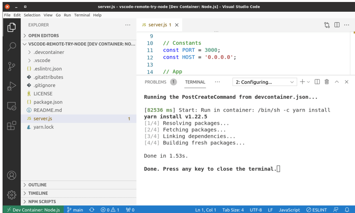
Figure 6.2 A Development Container Opened in VS Code
