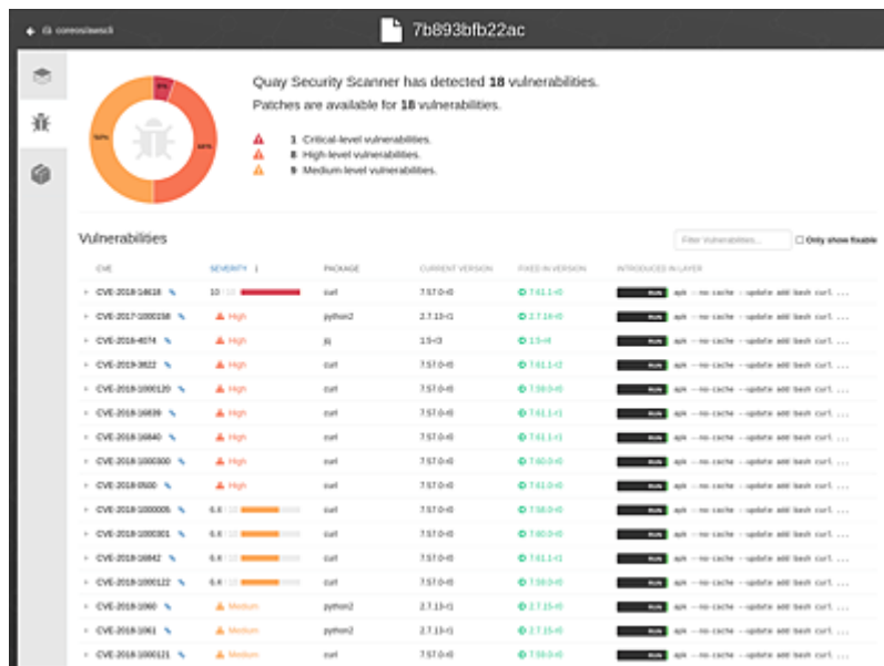
Figure 18.2 Security Scan for the coreos/awslcli Image in the Quay Repository
