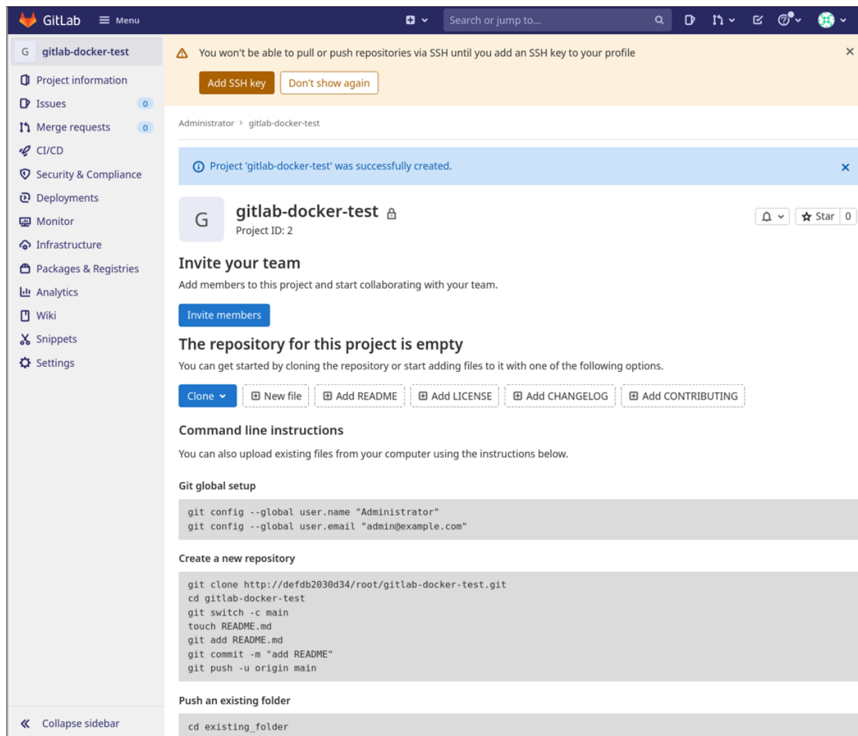
Figure 16.2 A New GitLab Project without Content
