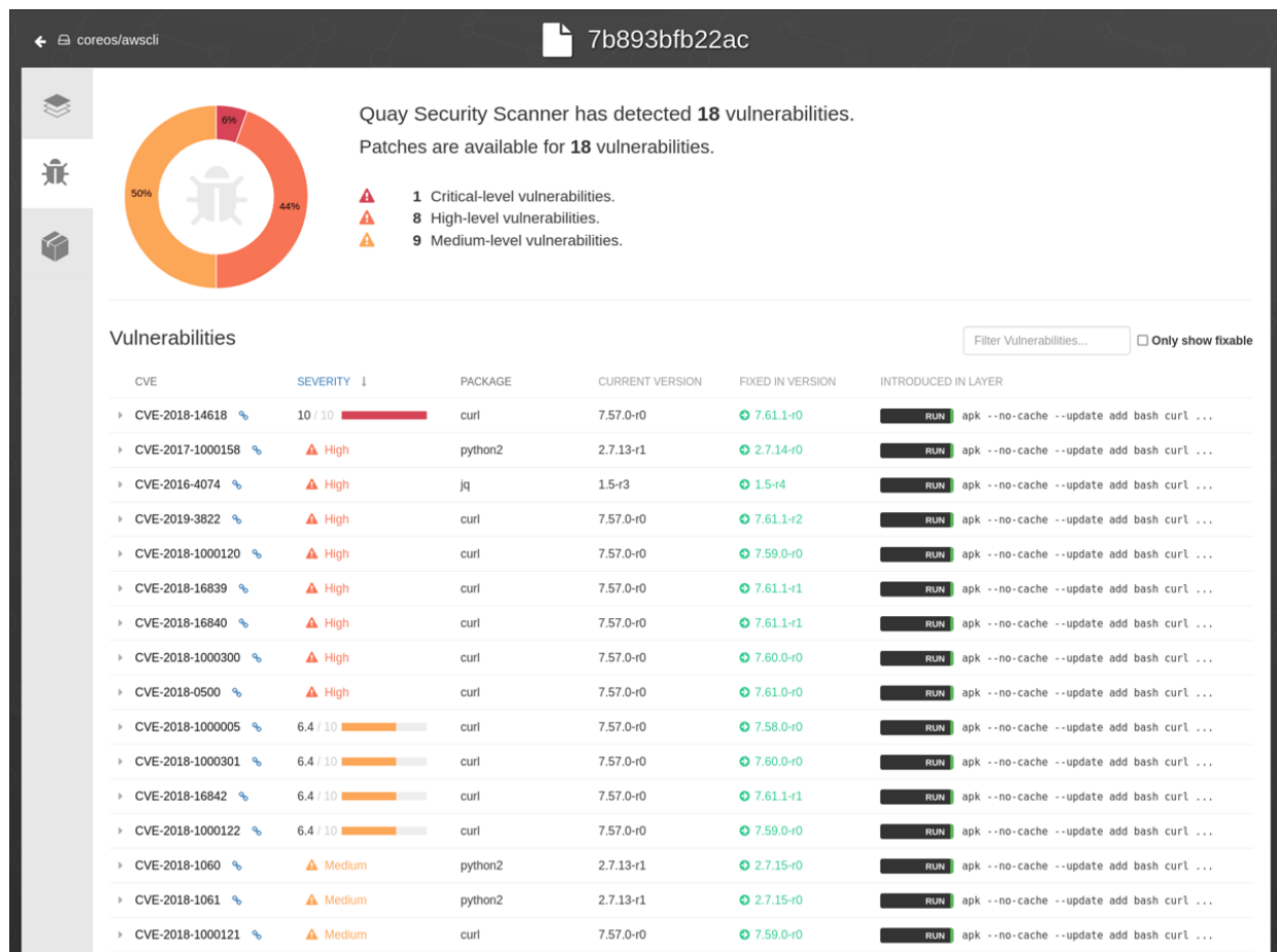
Figure 18.2 Security Scan for the coreos/awsccli Image in the Quay Repository
