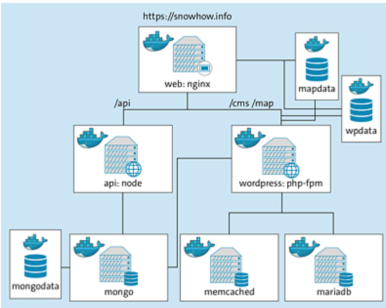
Figure 15.3 Docker Setup for the Conversion of the Web Application
