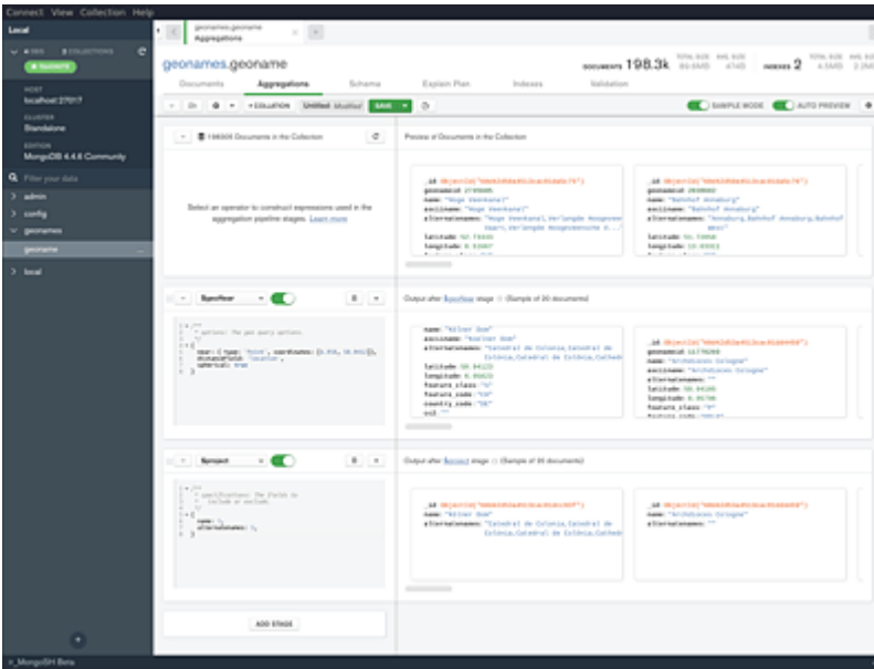
Figure 10.3 The MongoDB Compass Program When Creating an Aggregate Query
