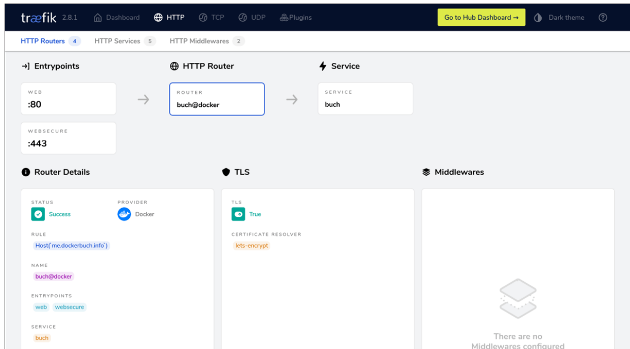
Figure 9.4 Traefik Dashboard with the New Router Details
