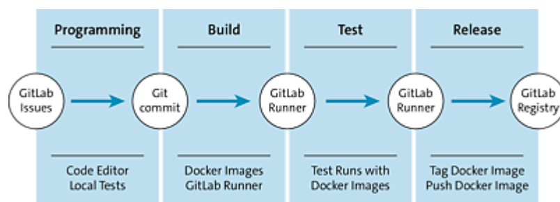
Figure 17.1 CI or CD Pipeline
