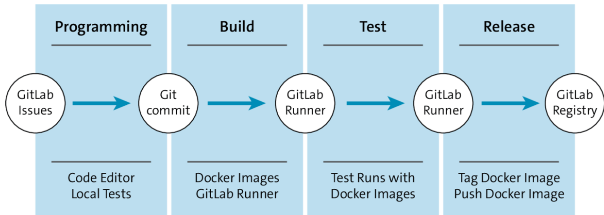
Figure 17.1 CI or CD Pipeline
