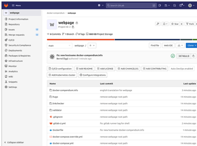
Figure 16.1 Overview of a GitLab Project
