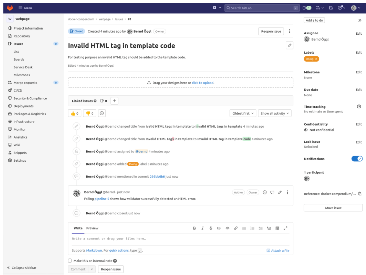
Figure 16.7 An Edited Ticket in GitLab
