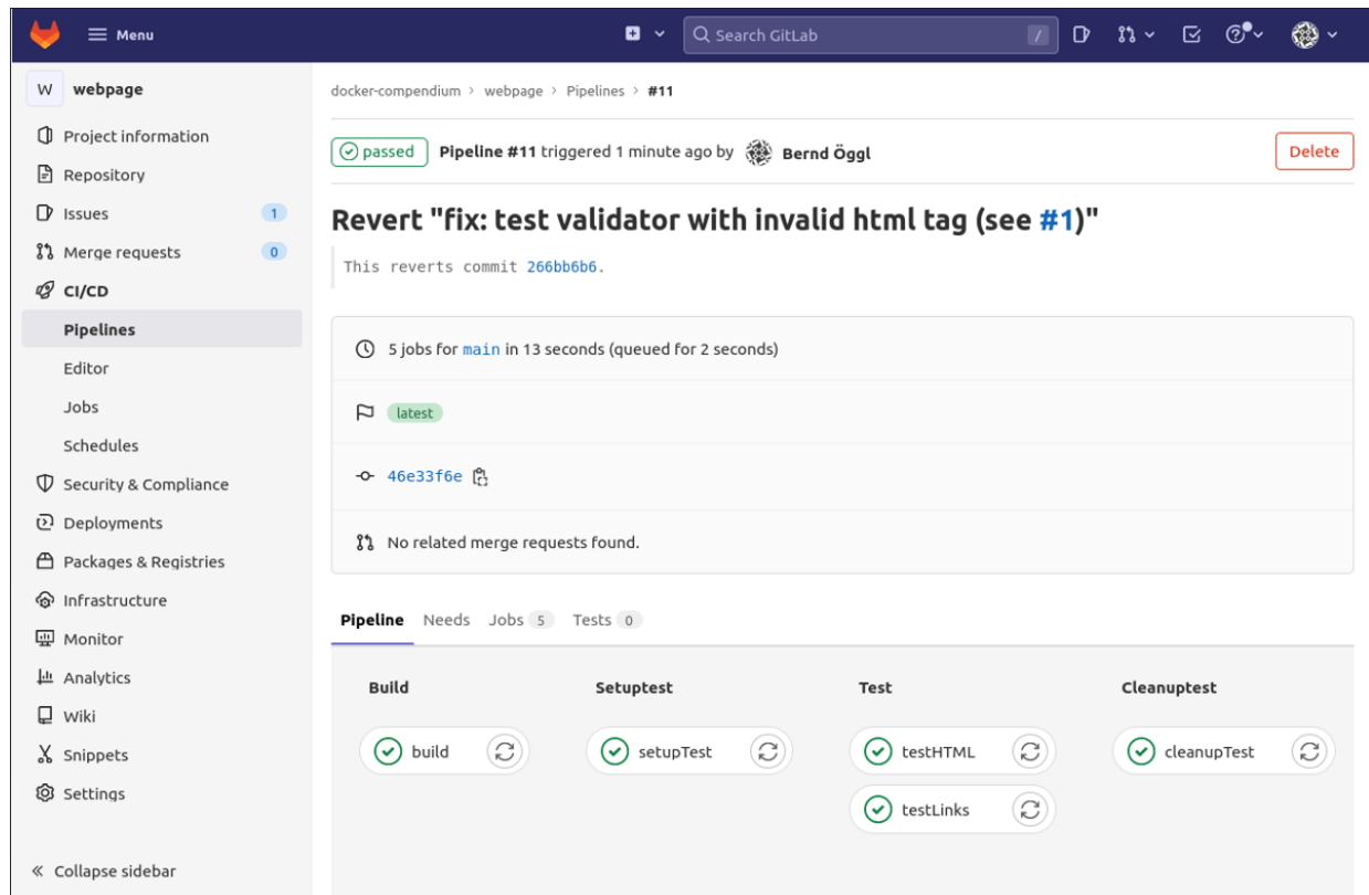
Figure 17.2 A Successful CI Pipeline in GitLab
