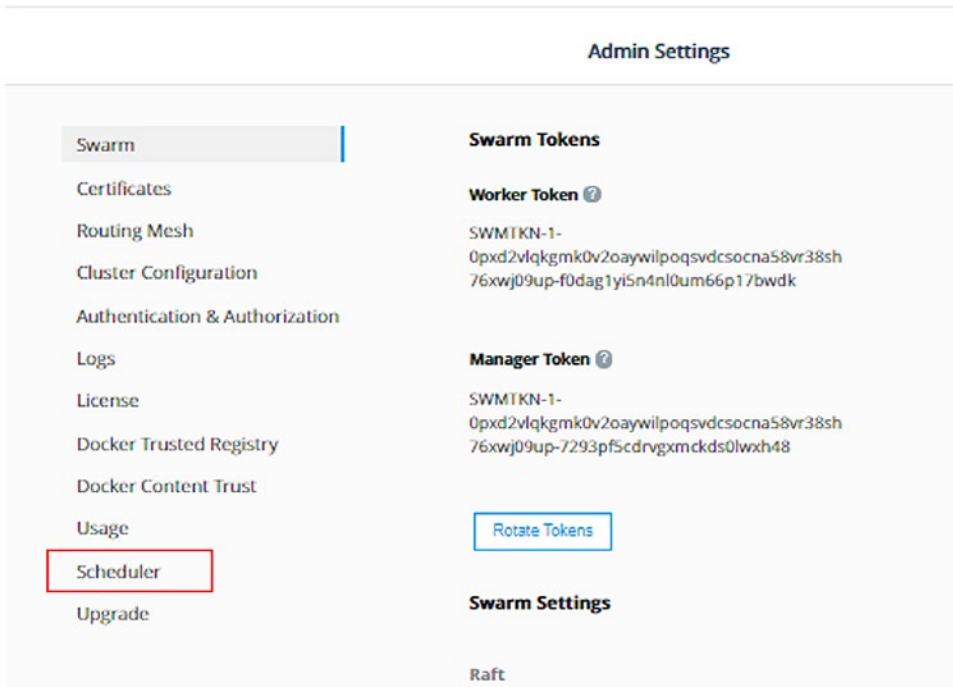
Figure 7-5. Scheduler
