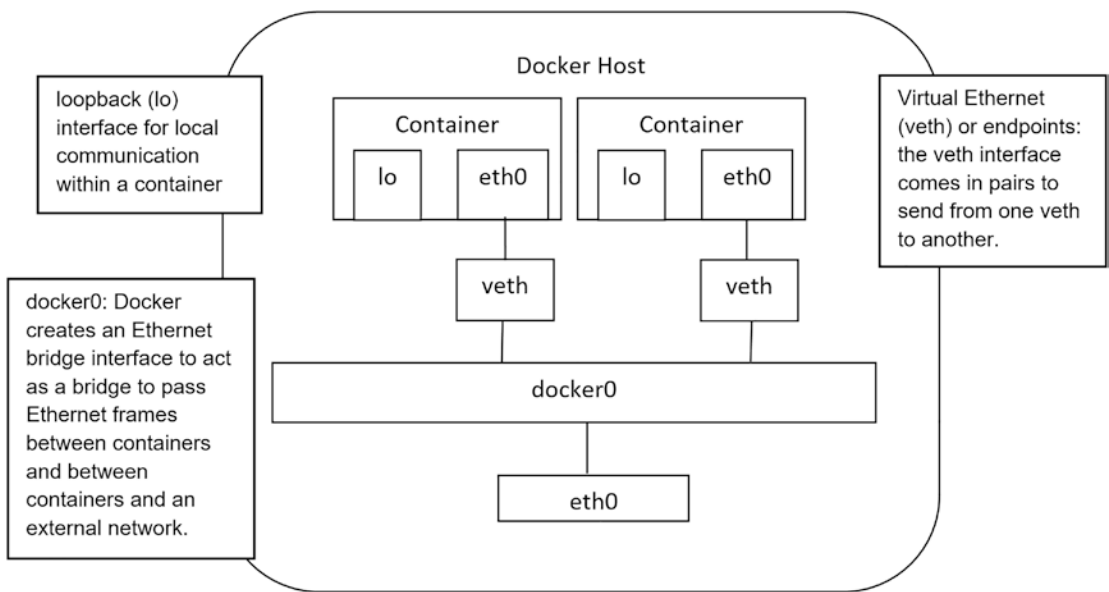
Figure 4-2. Bridge network
