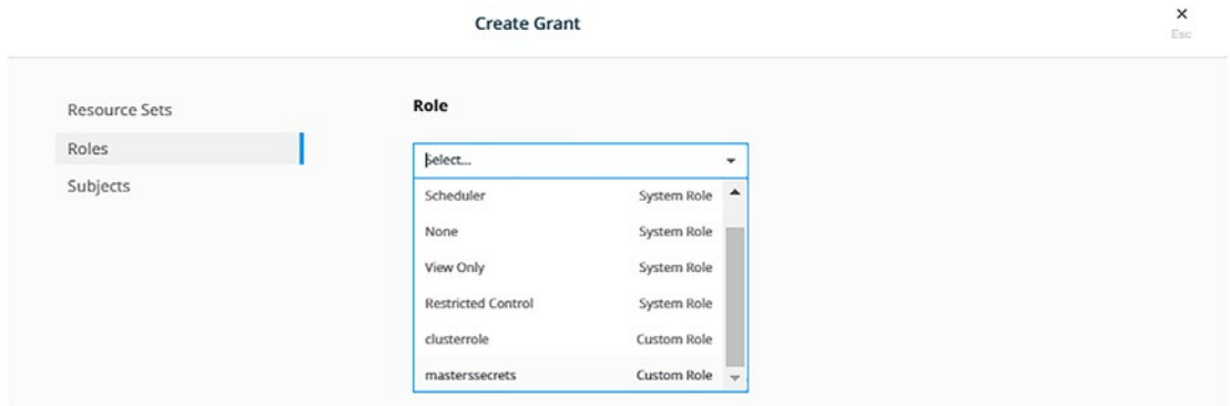
Figure 11-31. Select masterssecrets
