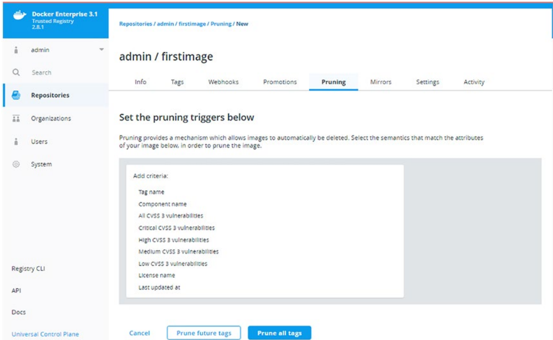
Figure 8-8. Pruning policies
