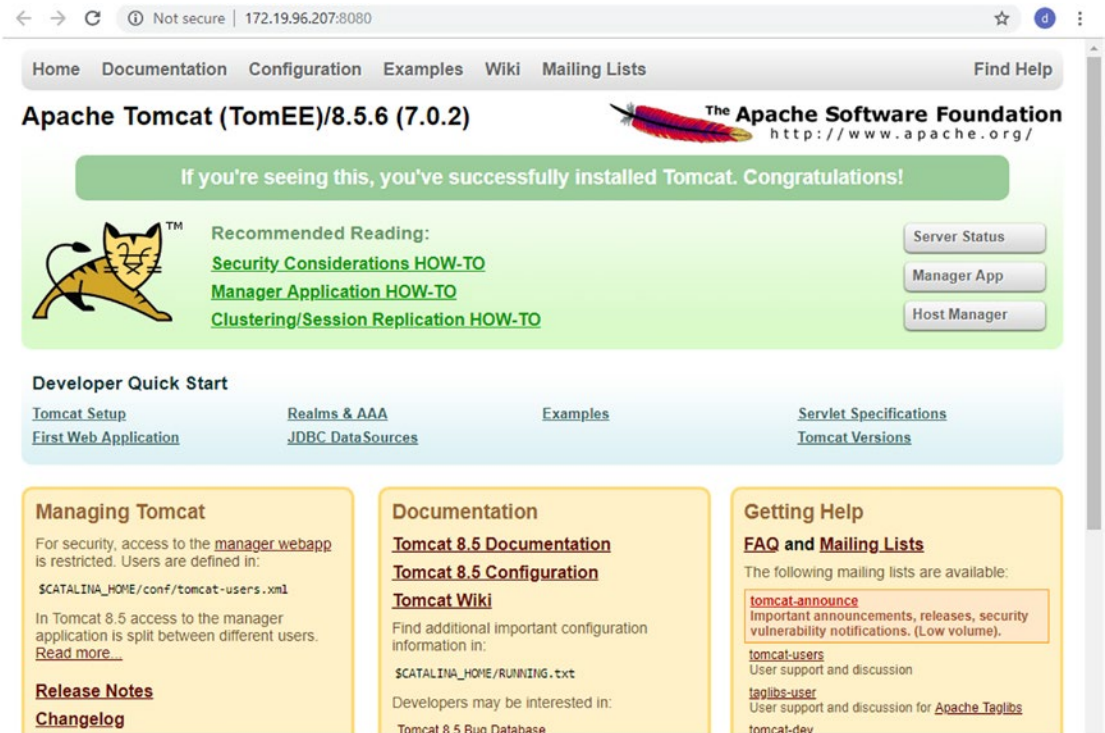
Figure 9-14. Tomcat service
