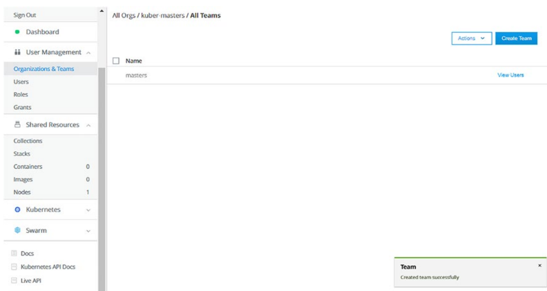
Figure 11-8. Team list
