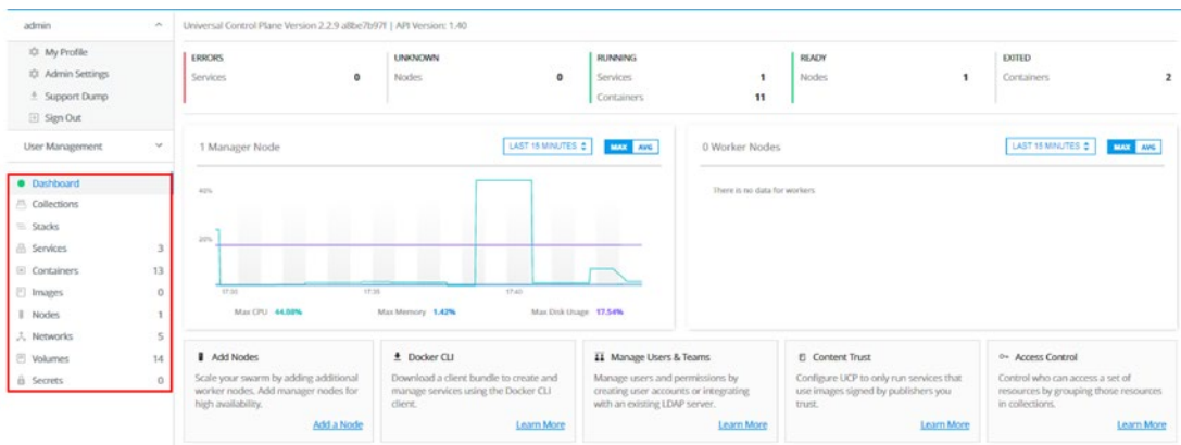
Figure 7-2. UCP version 2.2.9
