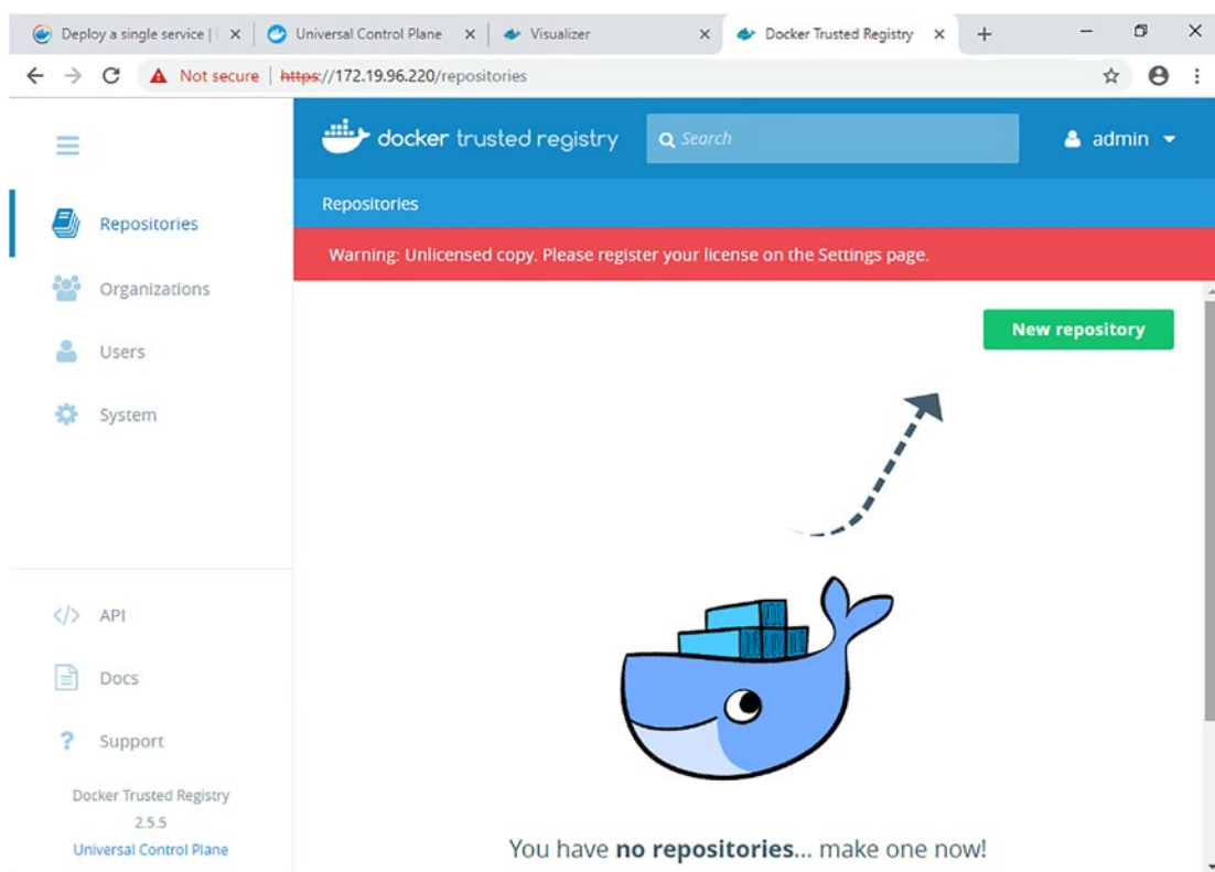
Figure 6-14. The DTR
