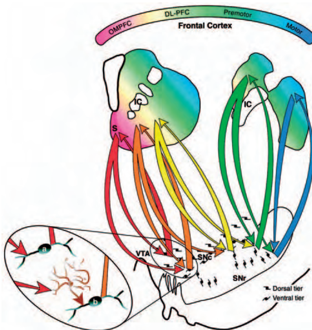
FIGURE 25.4 Ascending spirals of connectivity of the striatum to midbrain (downwards) and prefrontal cortex (upwards) (Reproduced from Haber et al. (2000) , with permission. VTA; Ventral tegmental area, S; shell of the nucleus accumbens, SNc/SNr; Substantia Nigra compacta/reticulata, IC; internal capsule, OMPFC; orbitomedial prefrontal cortex, DLPFC; dorsolateral prefrontal cortex).
