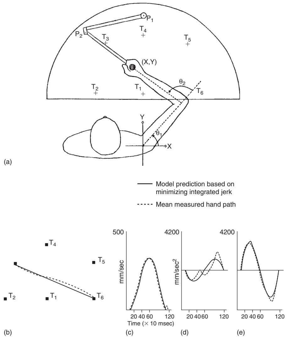
FIGURE 8.1 Example of a model of movement planning as optimization of a biomechanical constraint. (a) Subjects moved a manipulandum between various target positions (labeled T_1 , ..., T_6 ). (b) Hand path toward one example target. (c) Hand velocity. (d–e) Acceleration in the x (panel (d)) and y (panel (e)) directions. Dashed curves, mean measured hand path; solid curves, hand paths predicted by a model that minimized integrated jerk (rate of change of acceleration). The measured hand path shows a typical smoothly curved trajectory with a bell-shaped velocity profile. The minimum-jerk model (dashed curves) does a reasonable job of predicting movement kinematics. Reprinted from Flash and Hogan (1985) , with permission.
