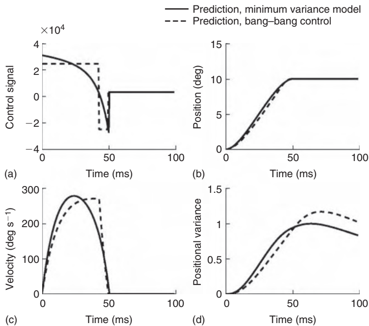
FIGURE 8.2 Predictions of a model of a 10°, 50-ms eye movement with signal-dependent noise. Dashed curves, the result of “bang-bang” control in which nearly maximum acceleration is applied throughout the movement until just prior to movement completion, at which point the eye is quickly brought to a stop; solid curves, movement achieving minimum positional variance at the end of the movement. The minimum-variance model predicts a bell-shaped velocity profile and results in substantially lower end-point variance. (a) Control signal; (b) position; (c) velocity; (d) positional variance.
