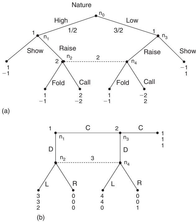
FIGURE 5.5 Imperfect information: (a) simple card game; (b) Selten's Horse. Figures 5.5(a) and 5.5(b) show some simple extensive form games with imperfect information. Again, the imperfection comes from the non-singleton information sets of players denoted by the dotted lines. Figure 5.5(a) shows a simple high-low card game where Nature deals a card to DM1, who sees if the card is high or low and can choose to show his card and win the pot if the card is high, or raise the dollar ante by another dollar. DM2 cannot see DM1's card (thus the information set) at n_2 and n_4 . Notice the irrelevance of order of the branches at the node, making it easier to depict the game and decision-makers' information. Figure 5.5(b) depicts Selten's Horse, where DM3 is uncertain if he is at n_2 or n_4 . This matters a lot to DM3, who prefers to move L at n_2 and R at n_3 . To solve this dilemma, DM3 must take into account the rational behavior of DM1 and DM2. Suppose DM3 believes that DM1 and DM2 may make small mistakes in implementing their strategy. A Nash Equilibrium which is still rational with respect to small mistakes is called trembling hand perfect. In the Horse, (C, C, \text{prop}(L) < (1/4)) is trembling hand perfect.
