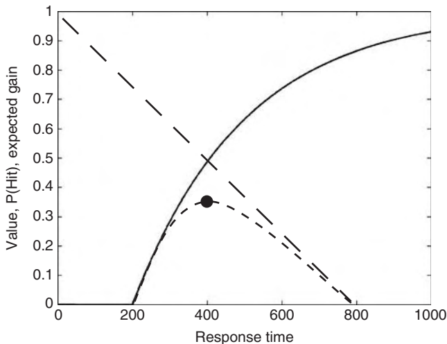
FIGURE 8.7 Calculation of expected gain in the experiment of Dean et al. (2007) . Subjects reached for a target on a display screen and were rewarded if they hit the target. The value of a hit on the target decreased linearly with movement duration (dashed line). Increased movement duration results in decreased movement endpoint variance, leading to an increased probability of a hit on the target (solid curve). The product of the value and probability of a hit equals expected value (dotted curve). The duration corresponding to maximum expected gain is indicated by the circle.
