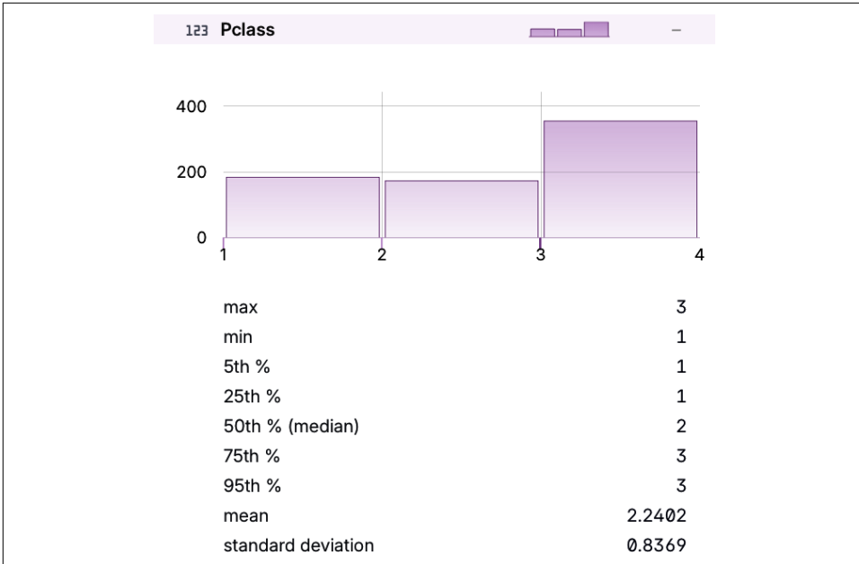
Figure 9-33. Histogram showing the number of passengers in each class
