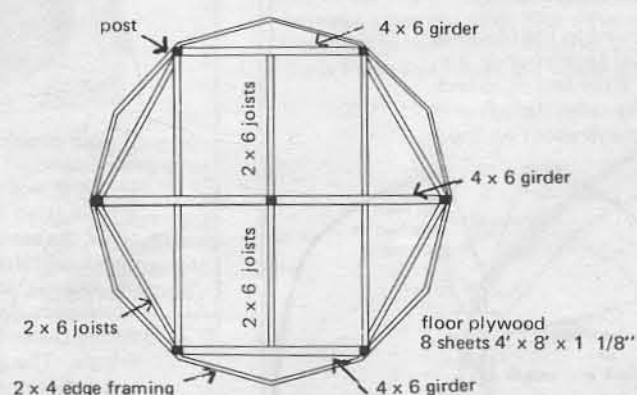
Floor framing plan.
