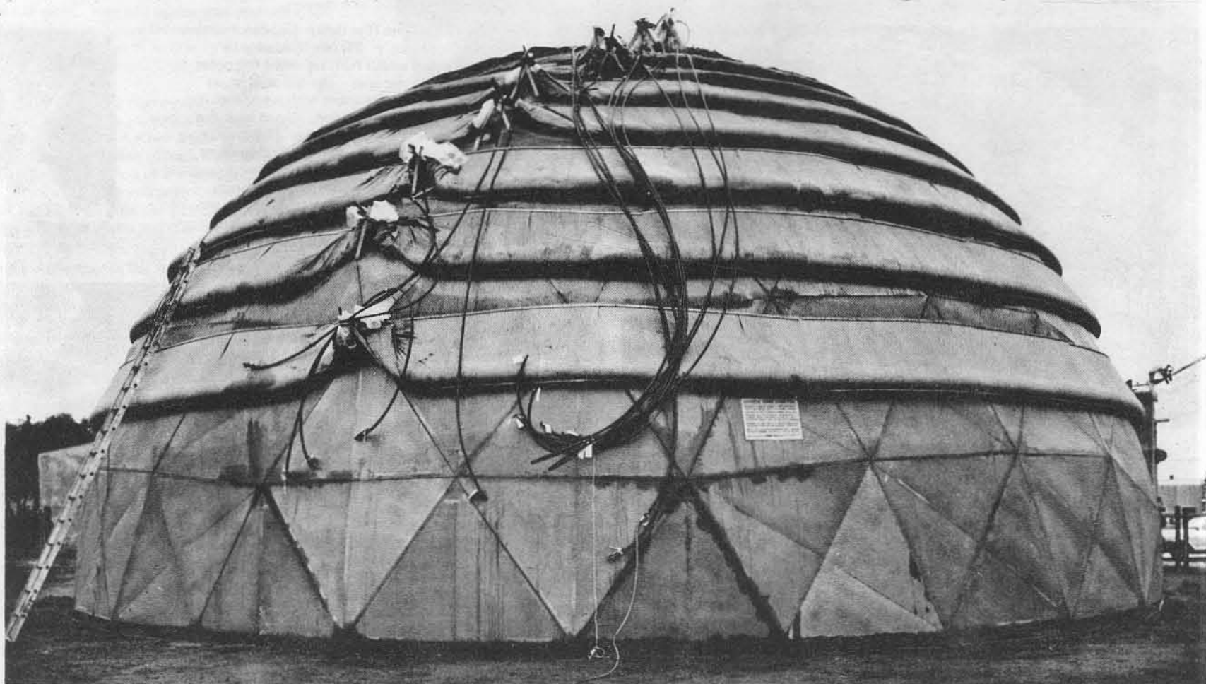
Test on plywood Pease dome by H. C. Nutting Co., Testing Engineers, Cincinnati, Ohio. Test data available from Pease Woodwork Co., Hamilton, Ohio. These domes
