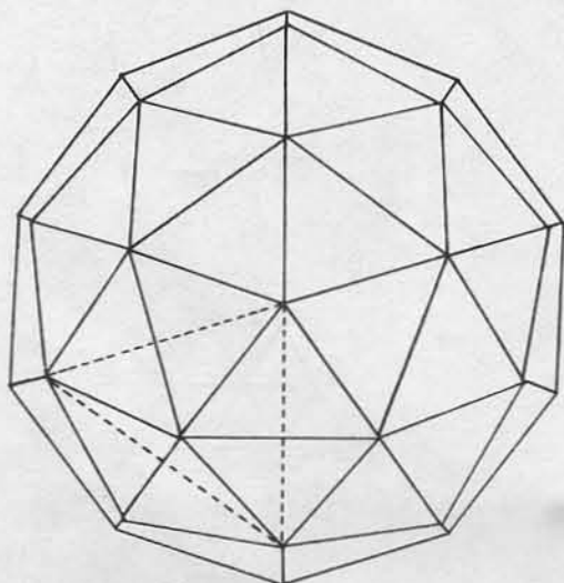
Top view of 2_v icos triacon. Icosa face dotted.
