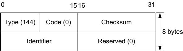
Figure 8-19 The MIPv6 Home Agent Address Discovery Request message contains an identifier that is returned in the response. It is sent to the Home Agents anycast address for the mobile node’s home prefix.
