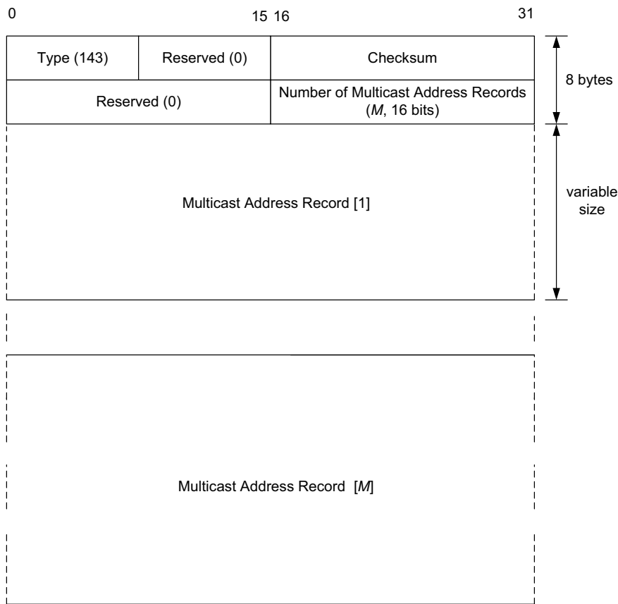
Figure 8-28 The MLDv2 Report message includes a vector of multicast address records.
