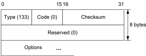
Figure 8-32 The ICMPv6 Router Solicitation message is very simple but ordinarily contains a Source Link-Layer Address option (unlike its ICMPv4 counterpart). It may also contain an MTU option if an unusual MTU value is in use on the link.
