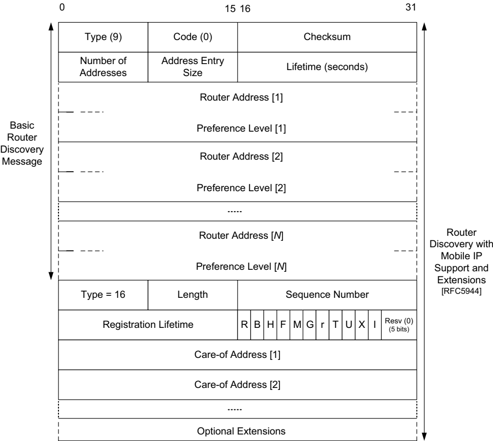
Figure 8-17 The ICMPv4 Router Advertisement message includes a list of IPv4 addresses of routers that can be used as default next hops. The preference level lets network operators arrange for some ordering of preferences to be applied with respect to the list (higher is more preferred). Mobile IPv4 [RFC5944] augments RA messages with extensions in order to advertise MIPv4 mobility agents and the prefix lengths of the advertised router addresses.
