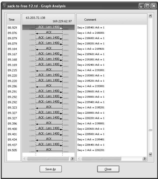
Figure 16-17 In Wireshark, the slow start behavior is apparent after a retransmission timeout. Each arriving ACK liberates two or three packets.
