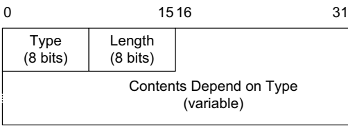
Figure 8-41 ND options are variable-length and begin with a common TLV arrangement. The Length field gives the total length of the option in 8-byte units (including the Type and Length fields).
