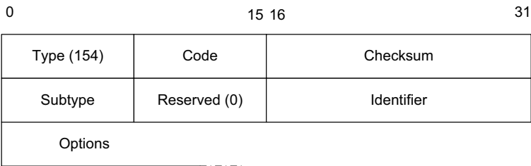
Figure 8-23 The common ICMPv6 message type used for FMIPv6 messages. The Code and Subtype fields give further information. Solicitation messages use code 0 and subtype 2 and may include the sender’s link-layer address and the link-layer address of its preferred next access point (if known) as options. Advertisements use codes 0–5 and subtype 3. The different code values indicate the presence of various options, whether the advertisement was solicited, if the prefix or router information has changed, and the handling of DHCP.
