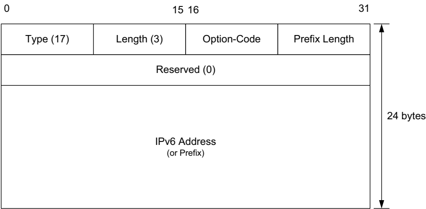
Figure 8-55 The IP Address/Prefix option used with FMIPv6. The option holds a prefix or IPv6 address of the next access router or care-of address used by a mobile node.
