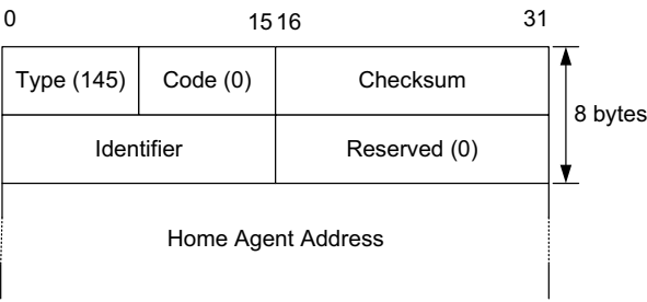
Figure 8-20 The MIPv6 Home Agent Address Discovery Reply message contains the identifier from the corresponding request and one or more addresses of a home agent willing to forward packets for the mobile node.
