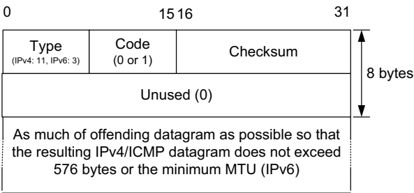
Figure 8-10 The ICMP Time Exceeded message format for ICMPv4 and ICMPv6. The message is standardized for both the TTL or hop count being exceeded (code 0) or the time for reassembling fragments exceeding some preconfigured threshold (code 1).
