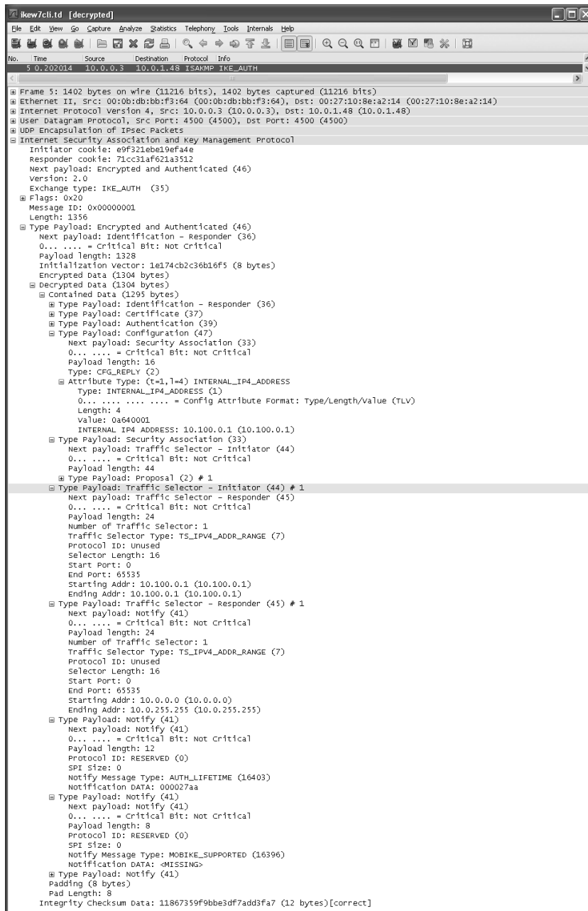
Figure 18-25 Completing the IKE_AUTH exchange, the responder produces an Encrypted/Authenticating data payload containing the following payloads: Identification responder (IDr), CERT, AUTH, CP(CFG_REPLY), SA, narrowed TSi and TSR, along with N(AUTH_LIFETIME), N(MOBIKE_SUPPORTED), and N(NO_ADDITIONAL_ADDRESSES). The first CHILD_SA can now commence.
