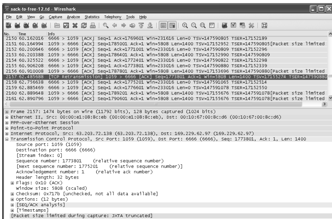
Figure 16-15 The sender experiences its first timeout when RTO = 1.57s . In this case, the sender declares the timeout to be spurious and undoes the modifications it made to its congestion control state.
