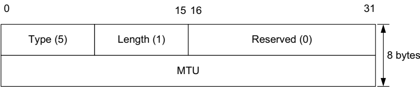
Figure 8-45 The MTU option includes the MTU to be used on the local link. This option is used with RA messages and is most useful if a nonstandard or unknown MTU is to be used.
