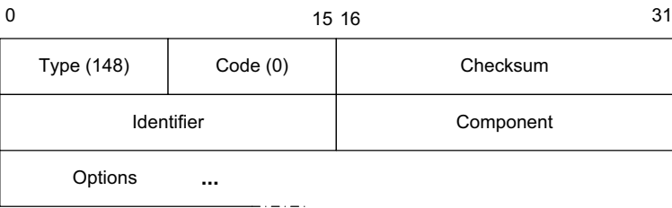
Figure 8-39 The Certification Path Solicitation message. The sender requests a particular certificate by position index, provided as the value of the Component field. The value 65535 indicates that all certificates in the path rooted at the identity given within an attached Trust Anchor option are desired.
