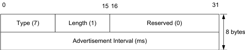
Figure 8-46 The Advertisement Interval gives the number of milliseconds between unsolicited multicast Router Advertisement messages.
