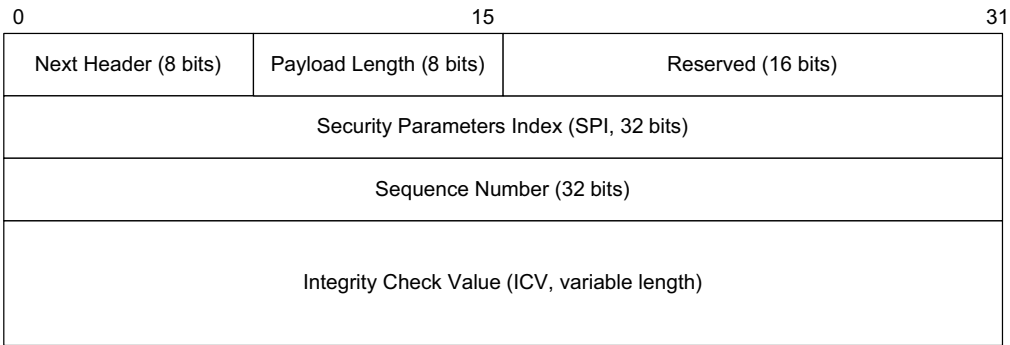
Figure 18-18 The IPsec AH is used to provide authentication and integrity protection for IPv4 and IPv6 datagrams in either transport or tunnel mode. The SPI value indicates which SA the AH belongs to. The Sequence Number field is used for countering replay attacks. The ICV provides a form of MAC over the immutable portions of the payload.
