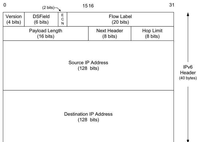
Figure 5-2 The IPv6 header is of fixed size (40 bytes) and contains 128-bit source and destination addresses. The Next Header field is used to indicate the presence and types of additional extension headers that follow the IPv6 header, forming a daisy chain of headers that may include special extensions or processing directives. Application data follows the header chain, usually immediately following a transport-layer header.
