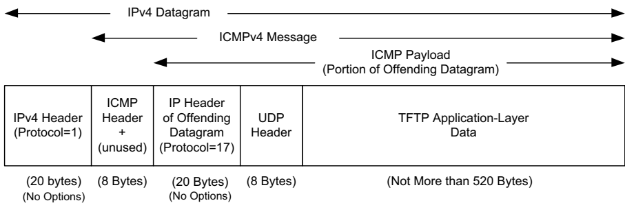
Figure 8-5 An ICMPv4 Destination Unreachable – Port Unreachable error message contains as much of the offending IPv4 datagram as possible such that the overall IPv4 datagram does not exceed 576 bytes. In this example, there is enough room to include the entire TFTP request message.
