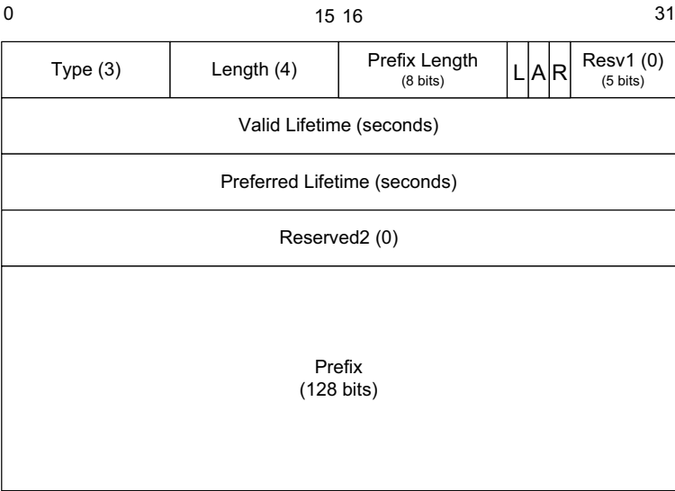
Figure 8-43 The Prefix Information option contains an IPv6 address prefix in use on the local network. It is used to provide hosts with prefixes for address autoconfiguration if the A bit field is set. The L bit field indicates that the prefix is acceptable for use in on-link determination. The R bit field is used to indicate that the included prefix is the entire global IPv6 address of the sending router.
