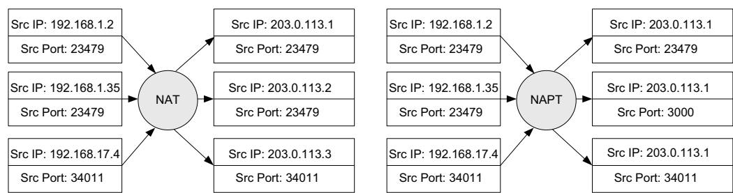
Figure 7-4 A basic IPv4 NAT (left) rewrites IP addresses from a pool of addresses and leaves port numbers unchanged. NAPT (right), also known as IP masquerading, usually rewrites address to a single address. NAPT must sometimes rewrite port numbers in order to avoid collisions. In this case, the second instance of port number 23479 was rewritten to use port number 3000 so that returning traffic for 192.168.1.2 could be distinguished from the traffic returning to 192.168.1.35.
