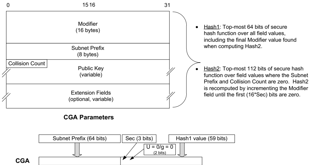
Figure 8-38 The SEND method for computing CGAs. The CGA parameters data structure is used as input to two cryptographic hash functions, Hash1 and Hash2. The Hash2 value must have (16*Sec) initial 0 bits, where Sec is a 3-bit parameter. The Modifier is changed until Hash2 computes appropriately. The resulting values are used to compute Hash1, which is combined with Sec and the subnet prefix to produce the CGA.
