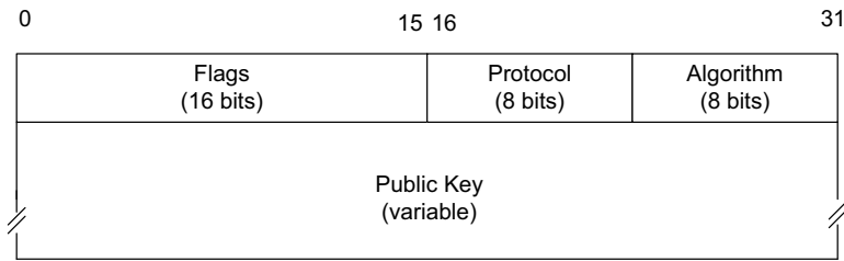
Figure 18-37 The RDATA portion of the DNSKEY RR contains a public key used only for DNSSEC. The Flags field includes a Zone Key indicator (bit 7), a Secure Entry Point indicator (bit 15), and Revoked indicator (bit 8). Generally, the zone key is set for all DNSSEC keys. If the advisory SEP bit is also set, the key is typically called a key signing key and is used for validating delegations to child zones. If not, the key is usually a zone signing key, has a shorter validity period, and is typically used to sign zone contents and not delegations. The included key is to be used with the algorithm specified in the Algorithm field.
