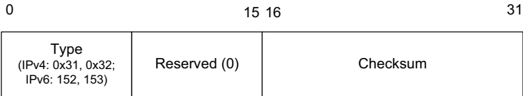
Figure 8-31 The ICMPv6 MRD Solicitation (ICMPv6 type 152; IGMP type 49) and Termination (ICMPv6 type 153; IGMP type 50) messages use a common format. MRD messages set the IPv6 Hop Limit field or IPv4 TTL field to 1 and include the Router Alert option. Solicitations are sent to the All Routers multicast address (IPv4, 224.0.0.2; IPv6, ff02::2).
