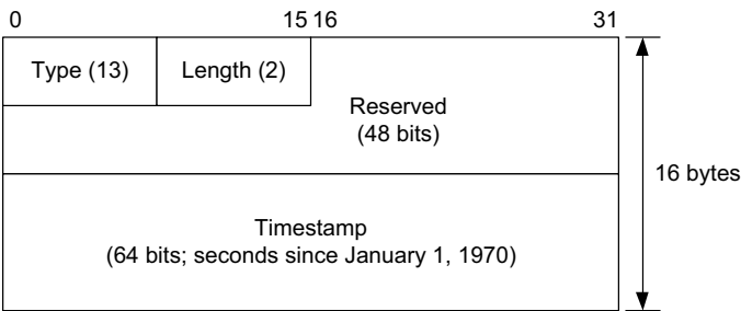
Figure 8-51 The Timestamp option used with SEND. The value encodes the number of seconds that have elapsed since January 1, 1970. It is used to guard against replay attacks.
