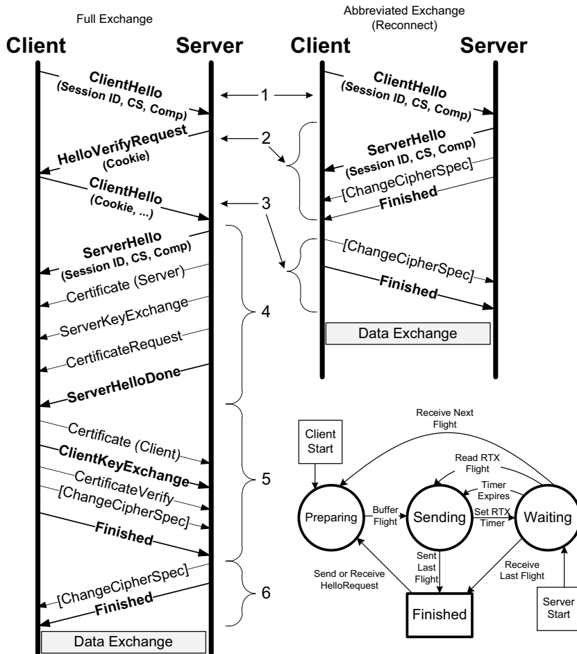
Figure 18-36 In DTLS, the possibility of lost datagrams must be handled. The initial full exchange (left) comprises six “flights” of information, each of which can be retransmitted. The DTLS abbreviated exchange (top right) uses only three and differs slightly from TLS. DTLS maintains a three-state finite state machine (bottom right) when processing the protocol.
