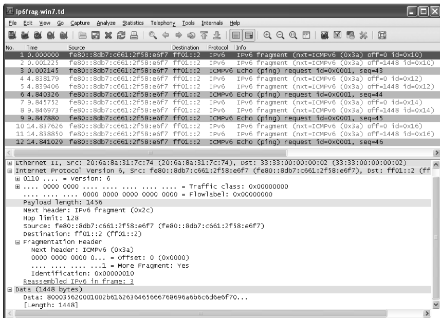
Figure 5-13 The ping program generates ICMPv6 packets (see Chapter 8) containing 3960 IPv6 payload bytes in this example. These packets are fragmented to produce three packet fragments, each of which is small enough to fit in the Ethernet MTU size of 1500 bytes.
