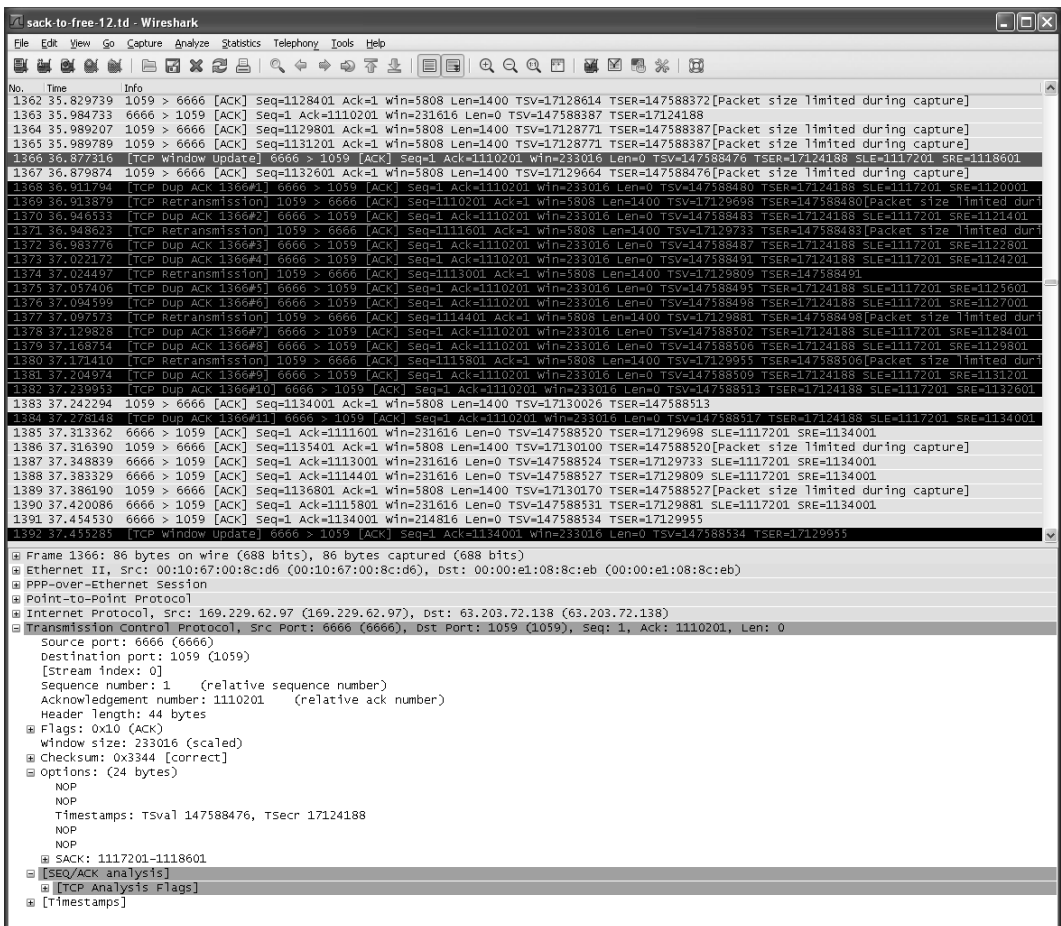
Figure 16-14 A Linux TCP sender enters the Disorder state upon receiving a duplicate ACK or an ACK with SACK information. Packets arriving while in this state trigger transmissions of new data. Subsequent duplicate ACKs (or presence of SACK information) place the sender into the Recovery state where retransmissions take place.
