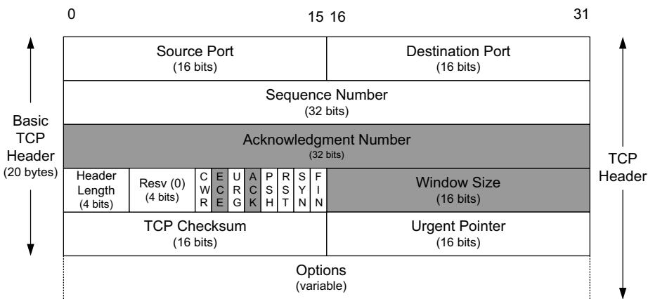
Figure 12-3 The TCP header. Its normal size is 20 bytes, unless options are present. The Header Length field gives the size of the header in 32-bit words (minimum value is 5). The shaded fields ( Acknowledgment Number , Window Size , plus ECE and ACK bits) refer to the data flowing in the opposite direction relative to the sender of this segment.
