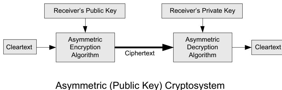
Figure 18-2 The unencrypted (cleartext) message is passed through an encryption algorithm to produce an encrypted (ciphertext) message. In a symmetric cryptosystem, the same (secret) key is used for encryption and decryption. In an asymmetric or public key cryptosystem, confidentiality is achieved by using the recipient's public key for encryption and private (secret) key for decryption.
