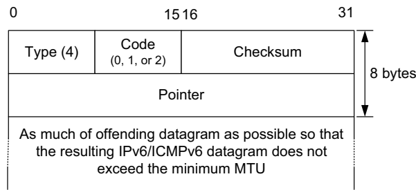
Figure 8-15 The ICMPv6 Parameter Problem message. The Pointer field gives the byte offset into the original datagram where an error was encountered. Code 0 indicates a bad header field. Code 1 indicates an unrecognized Next Header type, and Code 2 indicates that an unknown IPv6 option was encountered.
