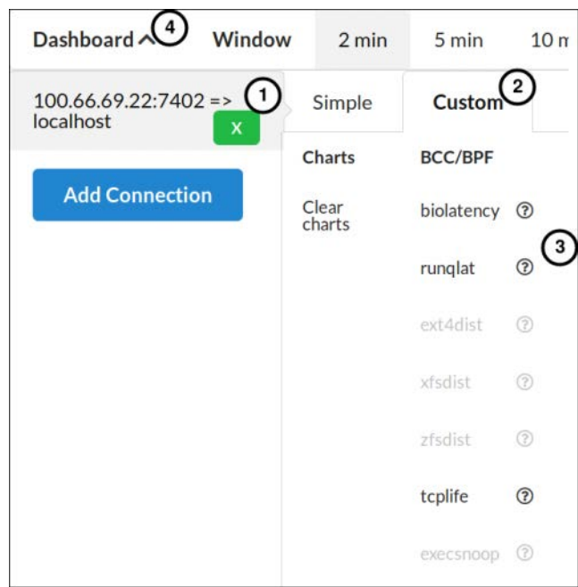
Figure 17-8 Vector selection of BCC/BPF tool
