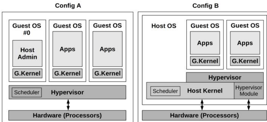
Figure 16-1 Common hypervisor configurations
