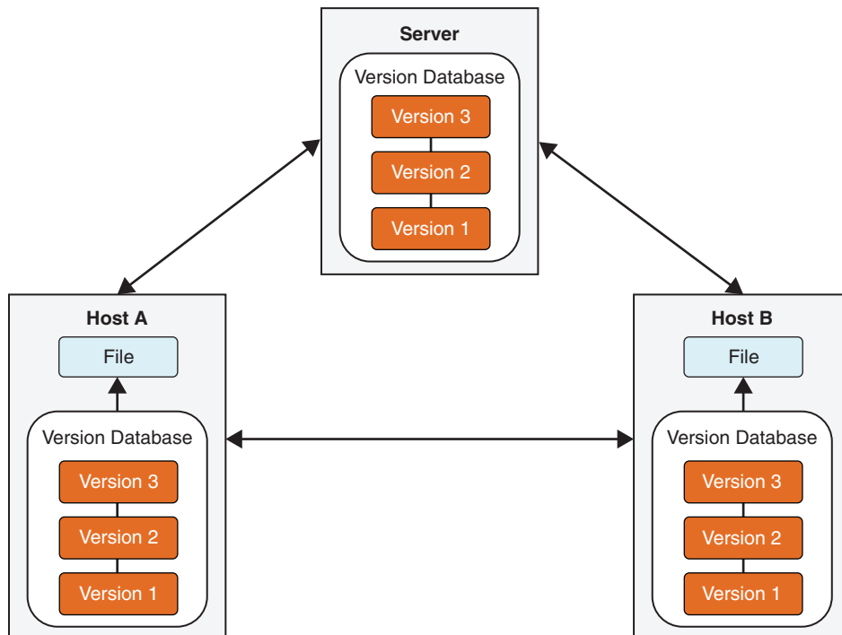
Figure 15-3 Third-generation version control software
