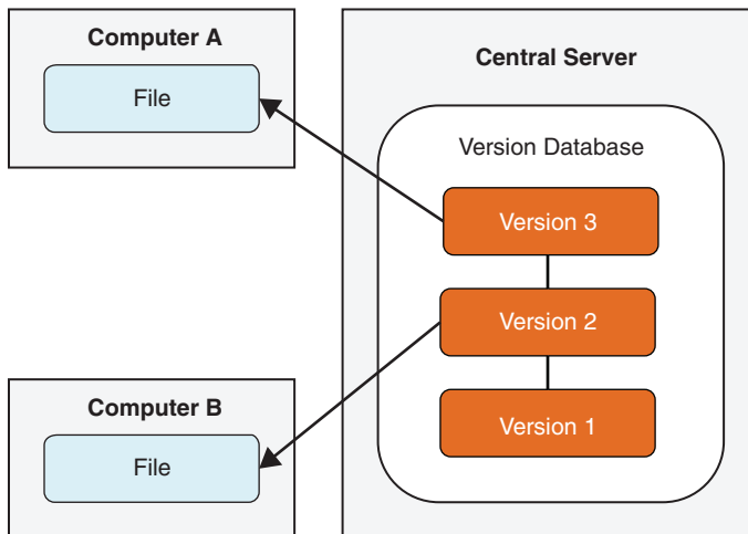
Figure 15-2 Second-generation version control software
