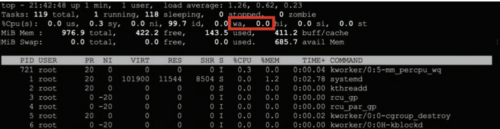
Figure 18-1 Example top command output showing the wa (wait time) value
