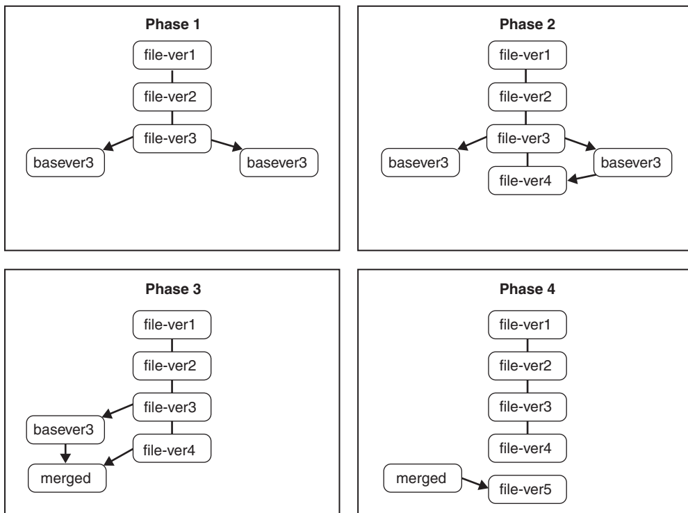
Figure 15-4 Second-generation merge and commit
