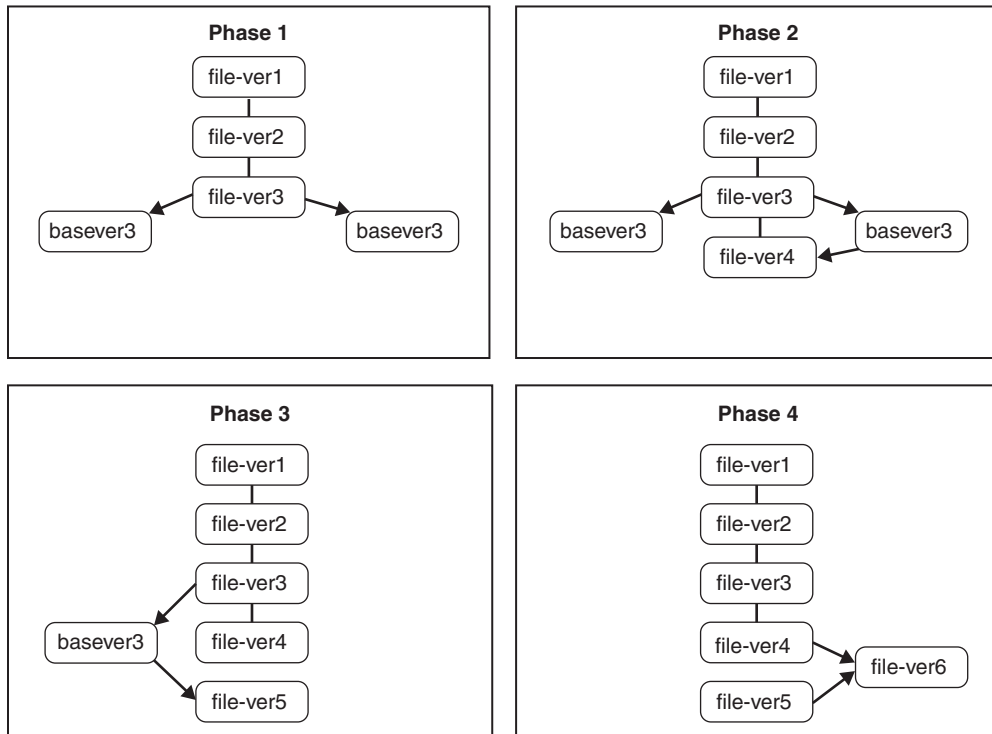
Figure 15-5 Third-generation commit and merge
