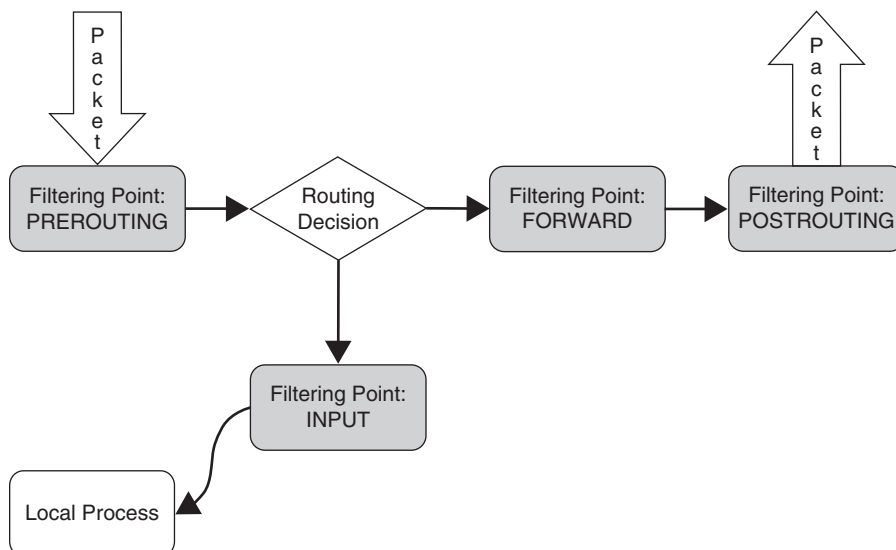
Figure 10-2 Packet filtering—routed packets
