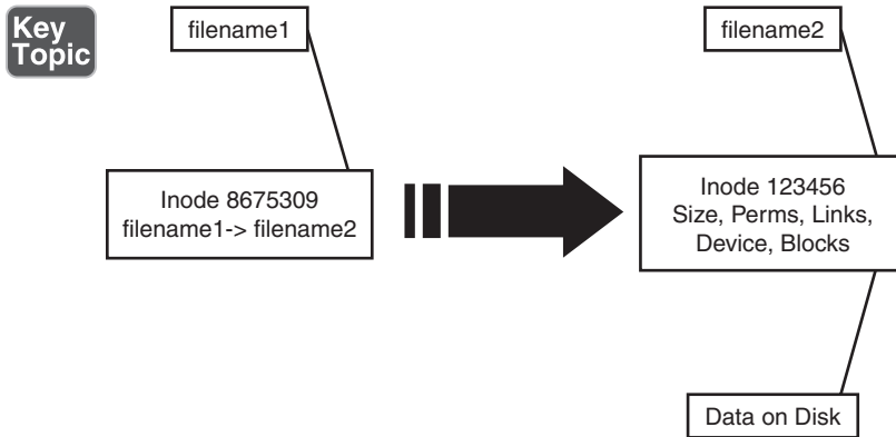
Figure 2-1 Symbolic link detail
