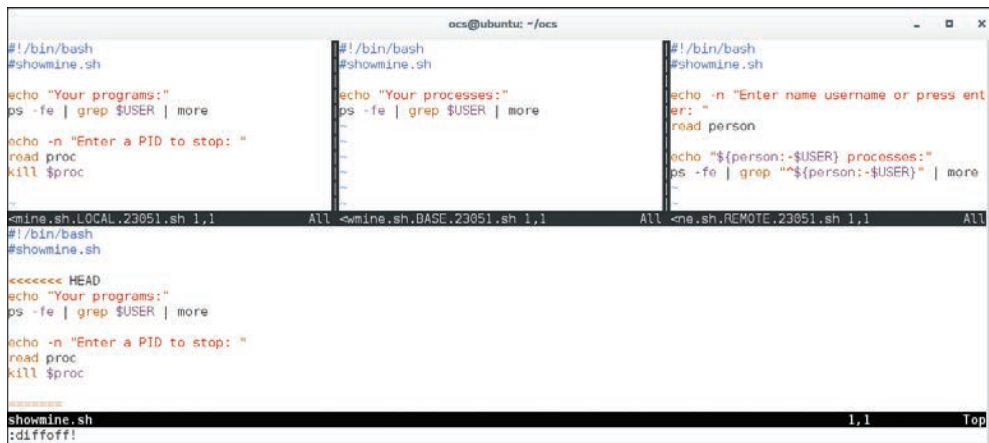
Figure 15-10 git mergetool using vimdiff
