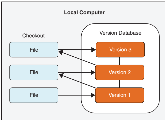
Figure 15-1 First-generation version control software
