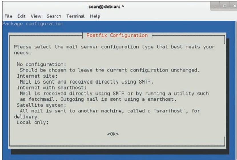
Figure 6-1 Reconfiguring Postfix with dpkg-reconfigure
