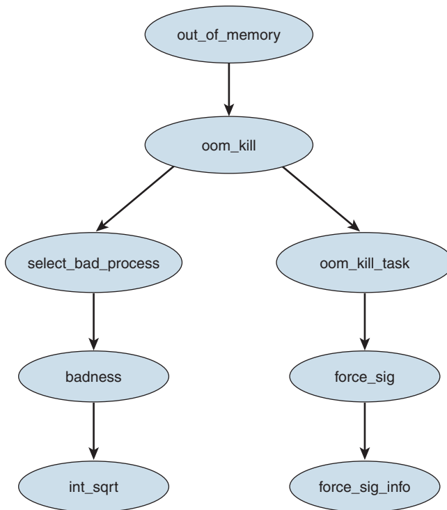
Figure 20-2 OOM Killer Process Diagram
