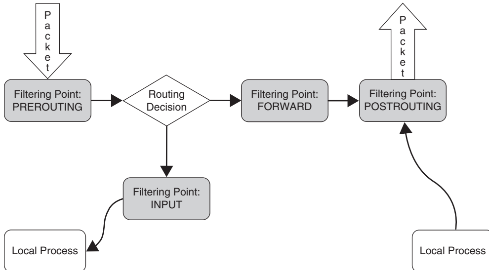
Figure 10-3 Packet filtering—outbound packets
